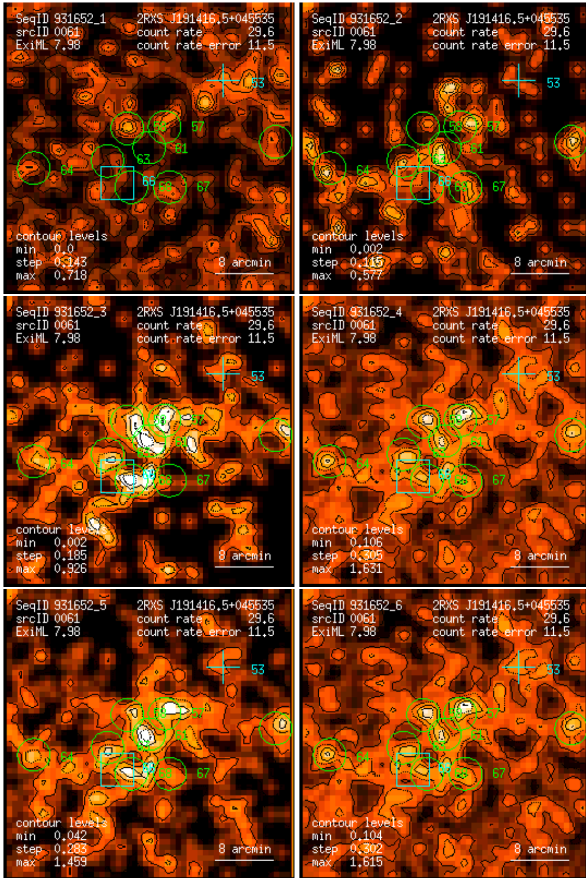
Figure 61: RASS 931652: detection 0061: band rate images, Gaussian filter: (1) PSPC channels 11 – 41, (2) 52 – 90, (3) 91 – 201, (4) 11 – 235, (5) 52 – 201, (6) 11 – 201. Broad band rates in counts/ks. Band rate contour levels in counts/ks/arcmin 2 .
