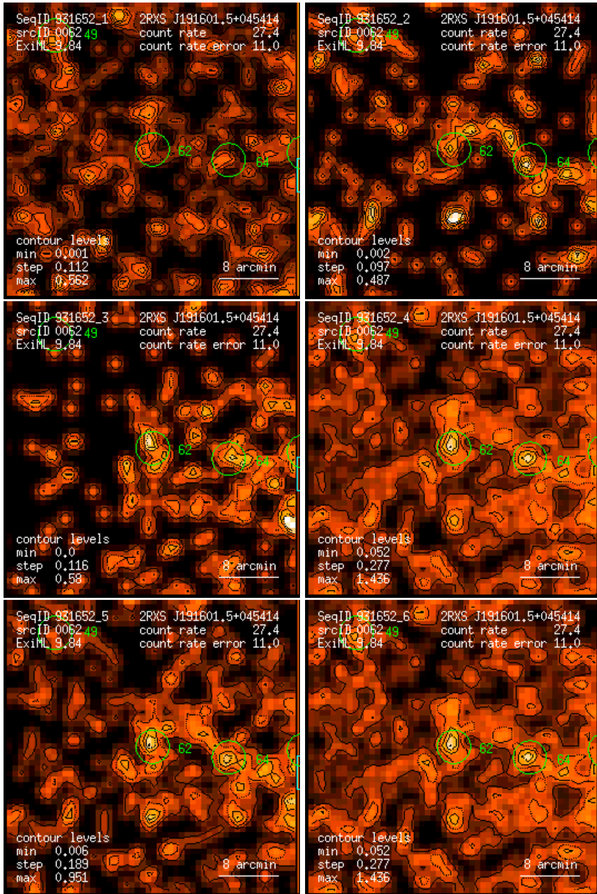
Figure 62: RASS 931652: detection 0062: band rate images, Gaussian filter: (1) PSPC channels 11 – 41, (2) 52 – 90, (3) 91 – 201, (4) 11 – 235, (5) 52 – 201, (6) 11 – 201. Broad band rates in counts/ks. Band rate contour levels in counts/ks/arcmin 2 .
