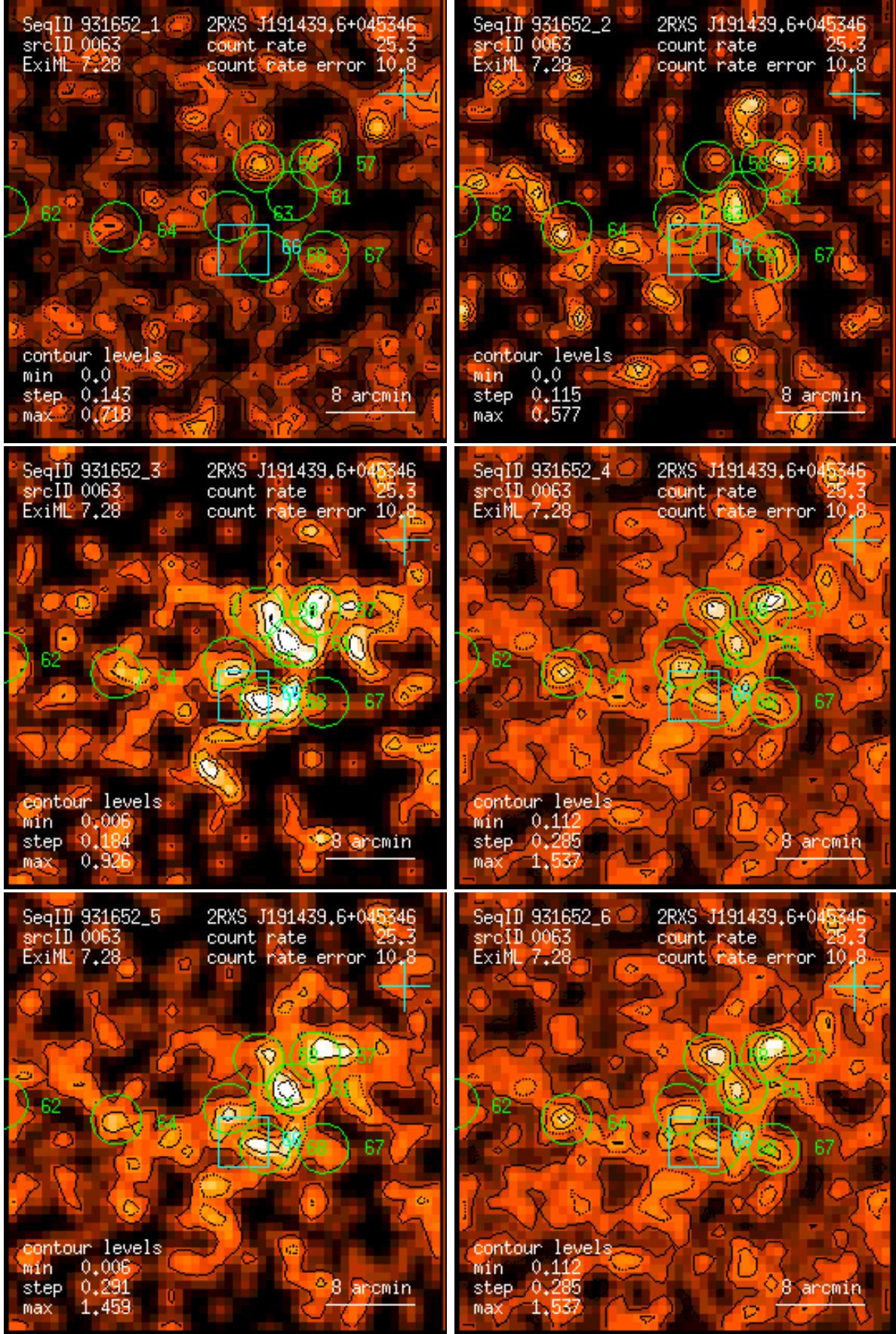
Figure 63: RASS 931652: detection 0063: band rate images, Gaussian filter: (1) PSPC channels 11 – 41, (2) 52 – 90, (3) 91 – 201, (4) 11 – 235, (5) 52 – 201, (6) 11 – 201. Broad band rates in counts/ks. Band rate contour levels in counts/ks/arcmin 2 .
