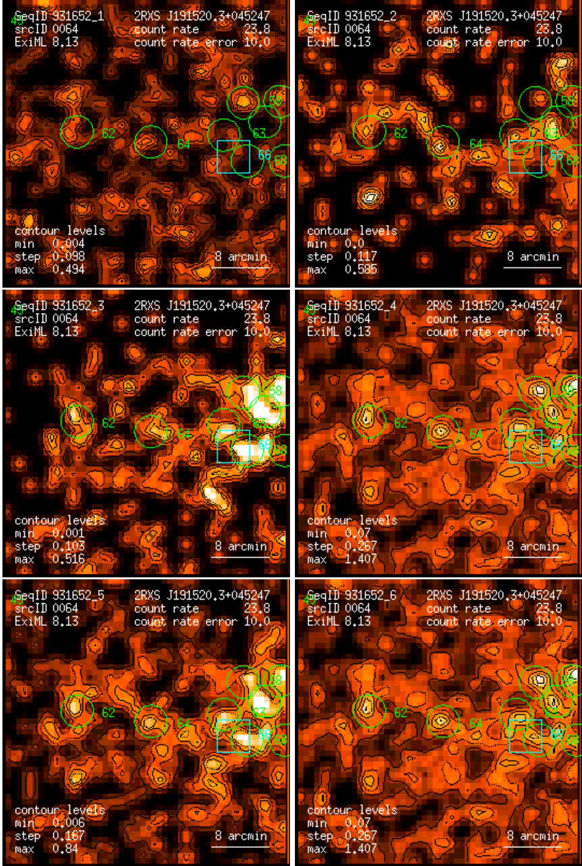
Figure 64: RASS 931652: detection 0064: band rate images, Gaussian filter: (1) PSPC channels 11 – 41, (2) 52 – 90, (3) 91 – 201, (4) 11 – 235, (5) 52 – 201, (6) 11 – 201. Broad band rates in counts/ks. Band rate contour levels in counts/ks/arcmin 2 .
