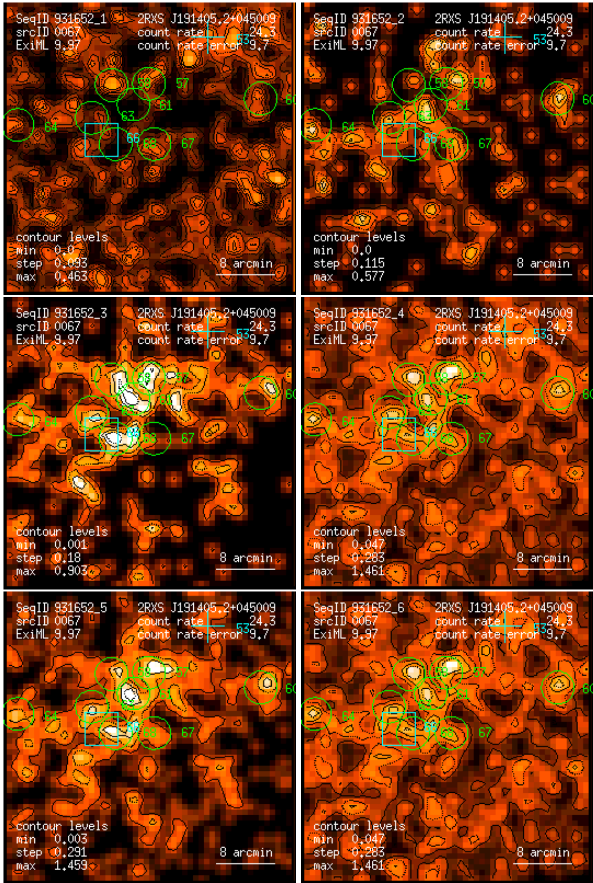
Figure 67: RASS 931652: detection 0067: band rate images, Gaussian filter: (1) PSPC channels 11 – 41, (2) 52 – 90, (3) 91 – 201, (4) 11 – 235, (5) 52 – 201, (6) 11 – 201. Broad band rates in counts/ks. Band rate contour levels in counts/ks/arcmin 2 .
