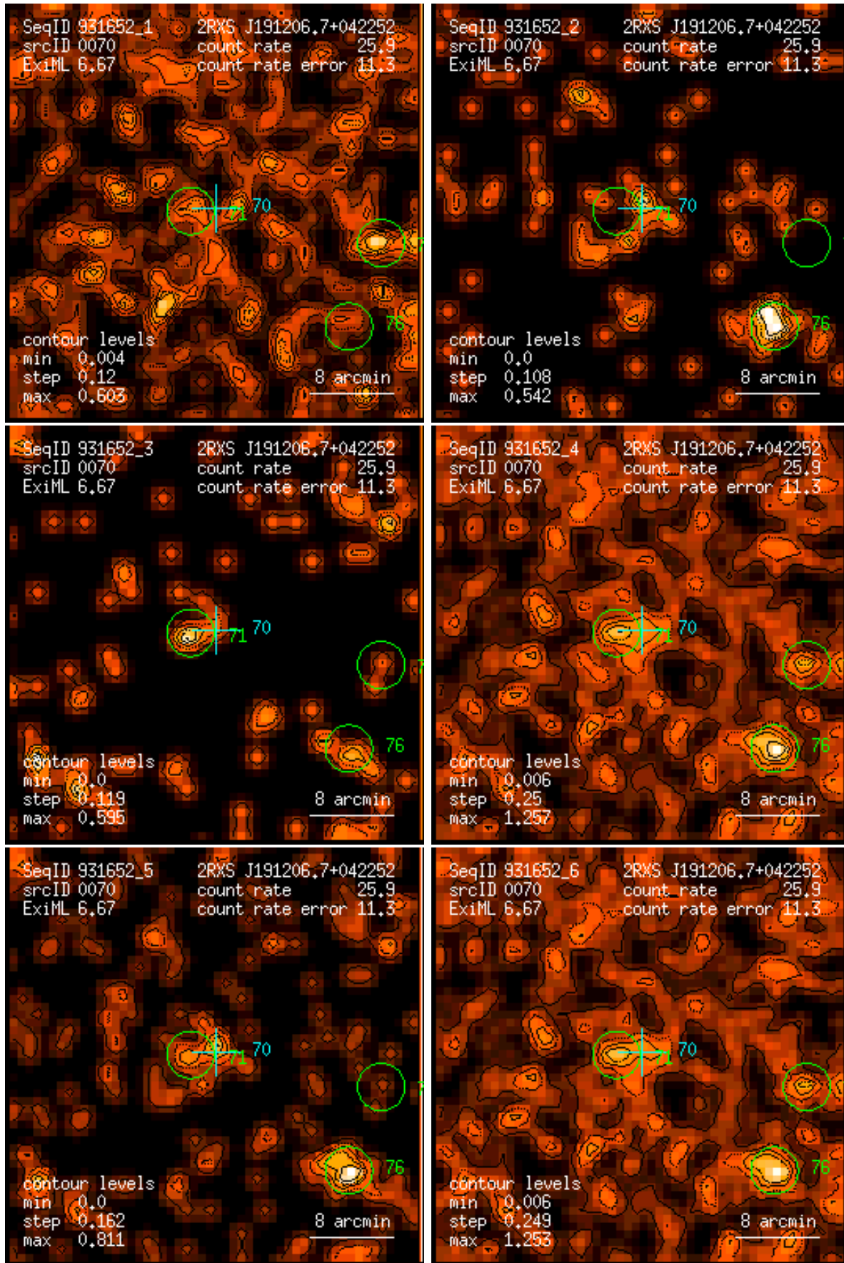
Figure 70: RASS 931652: detection 0070: band rate images, Gaussian filter: (1) PSPC channels 11 – 41, (2) 52 – 90, (3) 91 – 201, (4) 11 – 235, (5) 52 – 201, (6) 11 – 201. Broad band rates in counts/ks. Band rate contour levels in counts/ks/arcmin 2 .
