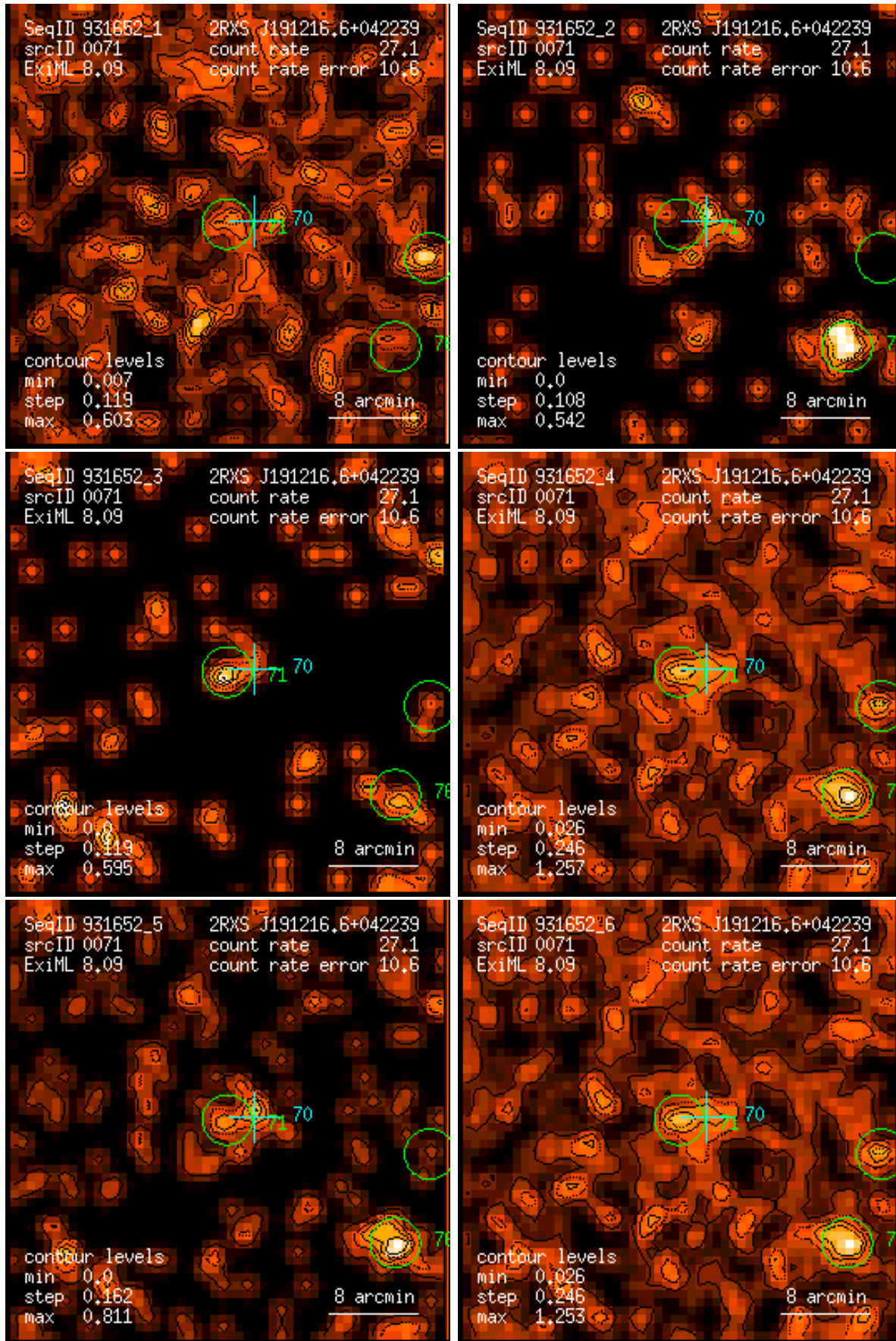
Figure 71: RASS 931652: detection 0071: band rate images, Gaussian filter: (1) PSPC channels 11 – 41, (2) 52 – 90, (3) 91 – 201, (4) 11 – 235, (5) 52 – 201, (6) 11 – 201. Broad band rates in counts/ks. Band rate contour levels in counts/ks/arcmin 2 .
