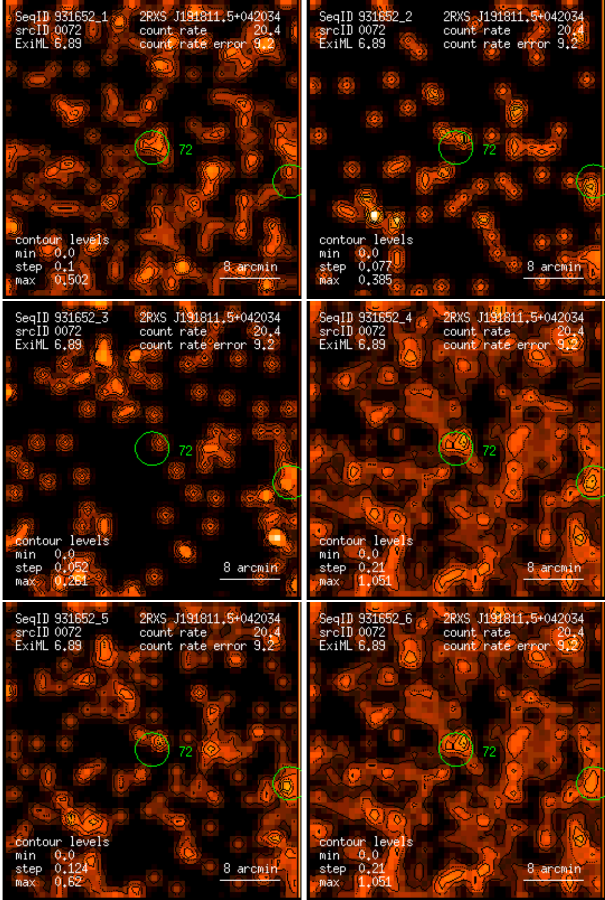
Figure 72: RASS 931652: detection 0072: band rate images, Gaussian filter: (1) PSPC channels 11 – 41, (2) 52 – 90, (3) 91 – 201, (4) 11 – 235, (5) 52 – 201, (6) 11 – 201. Broad band rates in counts/ks. Band rate contour levels in counts/ks/arcmin 2 .
