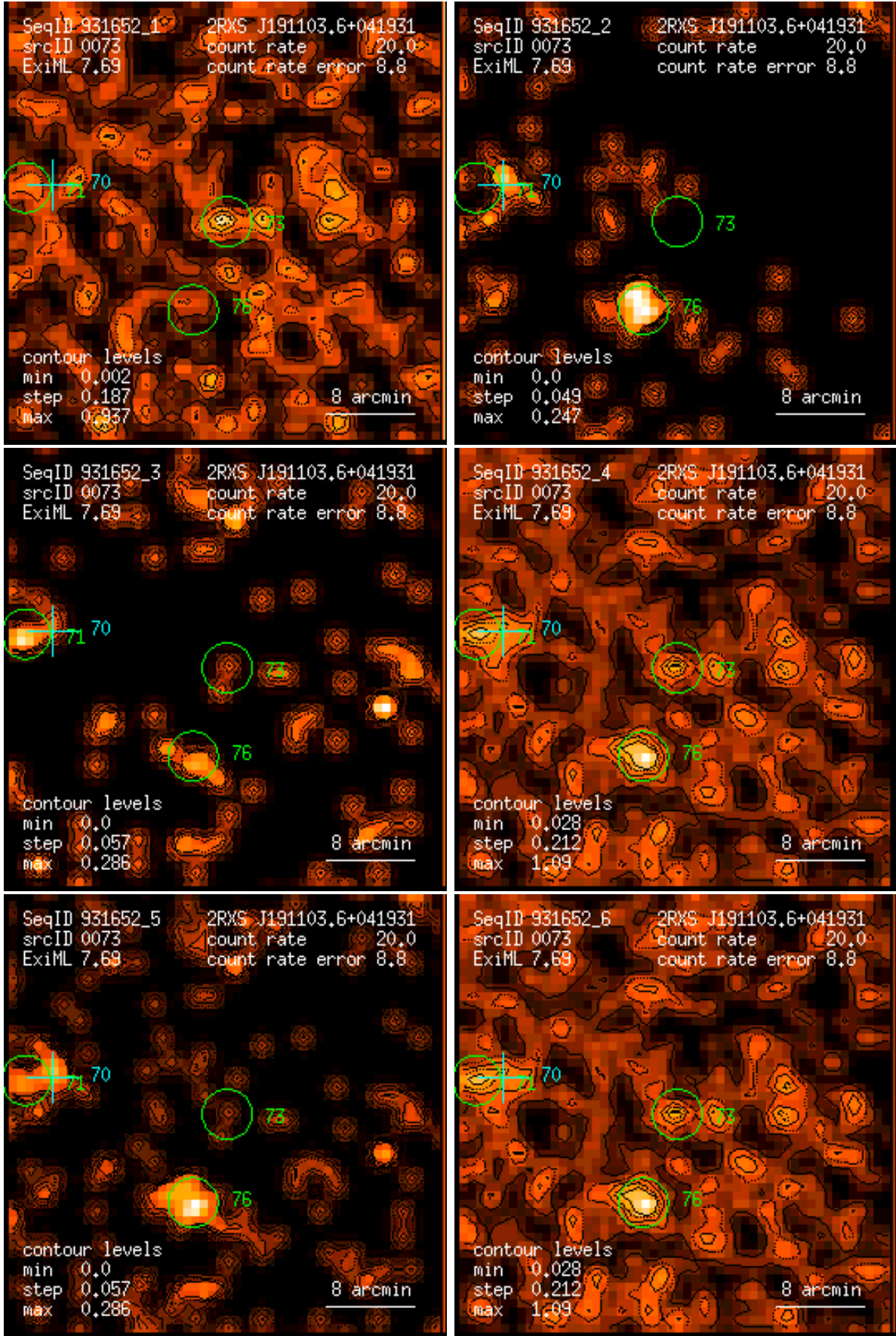
Figure 73: RASS 931652: detection 0073: band rate images, Gaussian filter: (1) PSPC channels 11 – 41, (2) 52 – 90, (3) 91 – 201, (4) 11 – 235, (5) 52 – 201, (6) 11 – 201. Broad band rates in counts/ks. Band rate contour levels in counts/ks/arcmin 2 .
