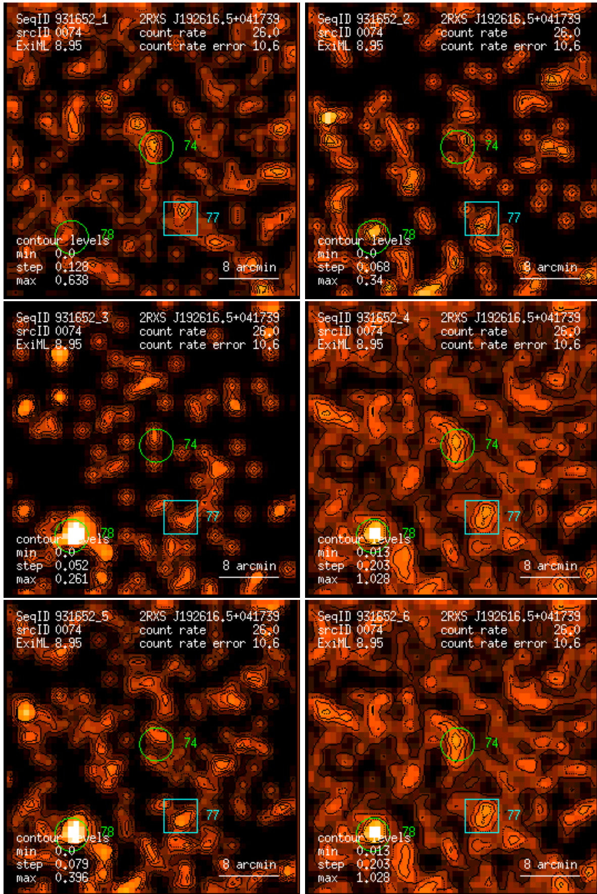
Figure 74: RASS 931652: detection 0074: band rate images, Gaussian filter: (1) PSPC channels 11 – 41, (2) 52 – 90, (3) 91 – 201, (4) 11 – 235, (5) 52 – 201, (6) 11 – 201. Broad band rates in counts/ks. Band rate contour levels in counts/ks/arcmin 2 .
