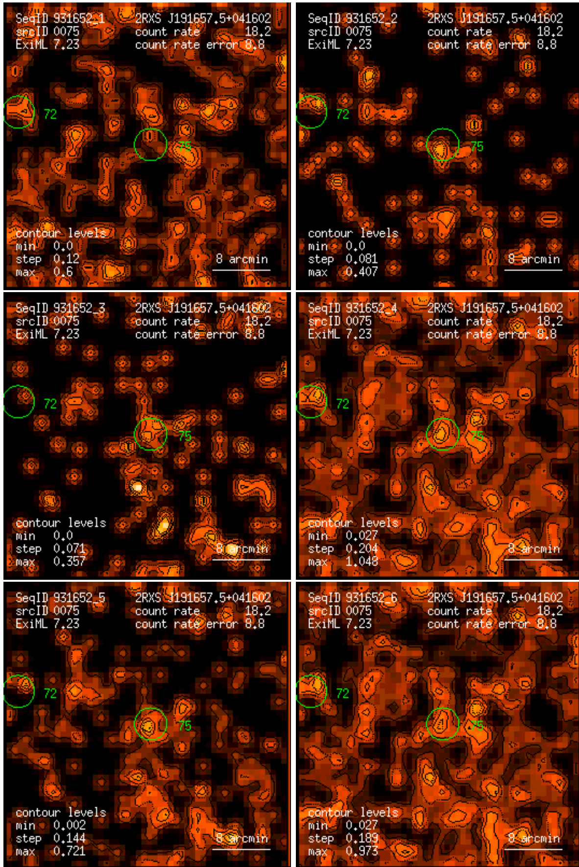
Figure 75: RASS 931652: detection 0075: band rate images, Gaussian filter: (1) PSPC channels 11 – 41, (2) 52 – 90, (3) 91 – 201, (4) 11 – 235, (5) 52 – 201, (6) 11 – 201. Broad band rates in counts/ks. Band rate contour levels in counts/ks/arcmin 2 .
