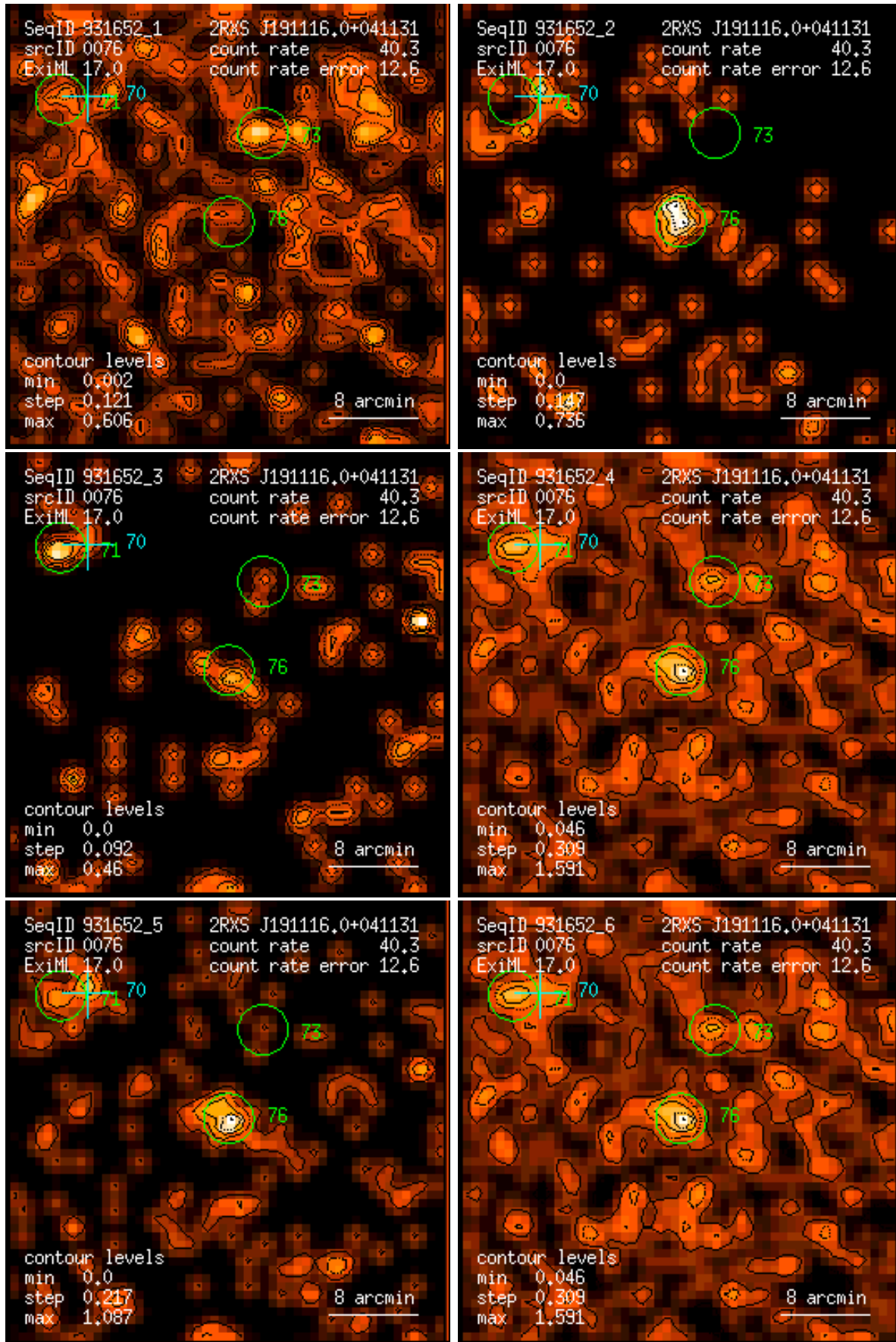
Figure 76: RASS 931652: detection 0076: band rate images, Gaussian filter: (1) PSPC channels 11 – 41, (2) 52 – 90, (3) 91 – 201, (4) 11 – 235, (5) 52 – 201, (6) 11 – 201. Broad band rates in counts/ks. Band rate contour levels in counts/ks/arcmin 2 .
