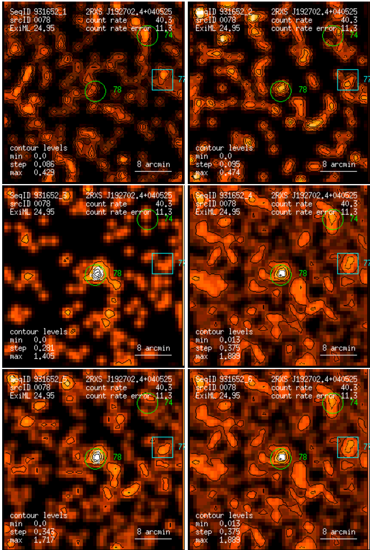
Figure 78: RASS 931652: detection 0078: band rate images, Gaussian filter: (1) PSPC channels 11 – 41, (2) 52 – 90, (3) 91 – 201, (4) 11 – 235, (5) 52 – 201, (6) 11 – 201. Broad band rates in counts/ks. Band rate contour levels in counts/ks/arcmin 2 .
