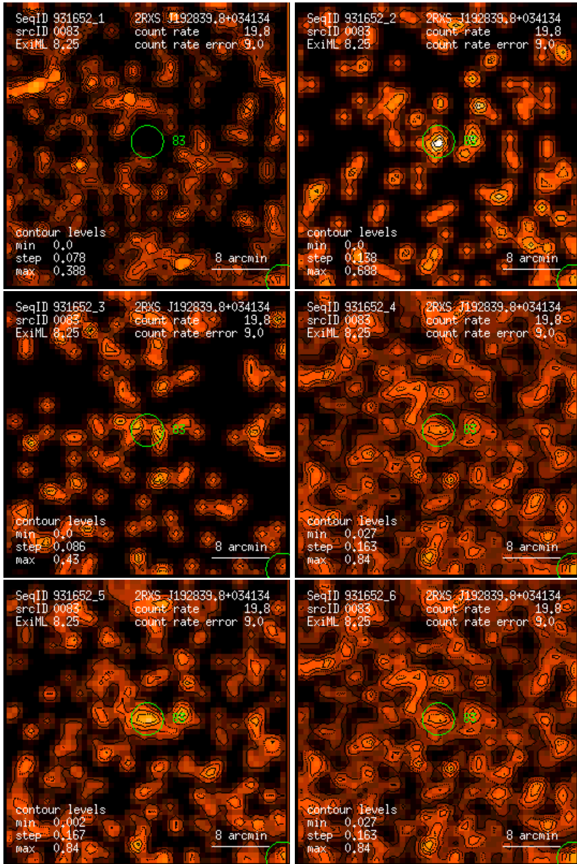
Figure 83: RASS 931652: detection 0083: band rate images, Gaussian filter: (1) PSPC channels 11 – 41, (2) 52 – 90, (3) 91 – 201, (4) 11 – 235, (5) 52 – 201, (6) 11 – 201. Broad band rates in counts/ks. Band rate contour levels in counts/ks/arcmin 2 .
