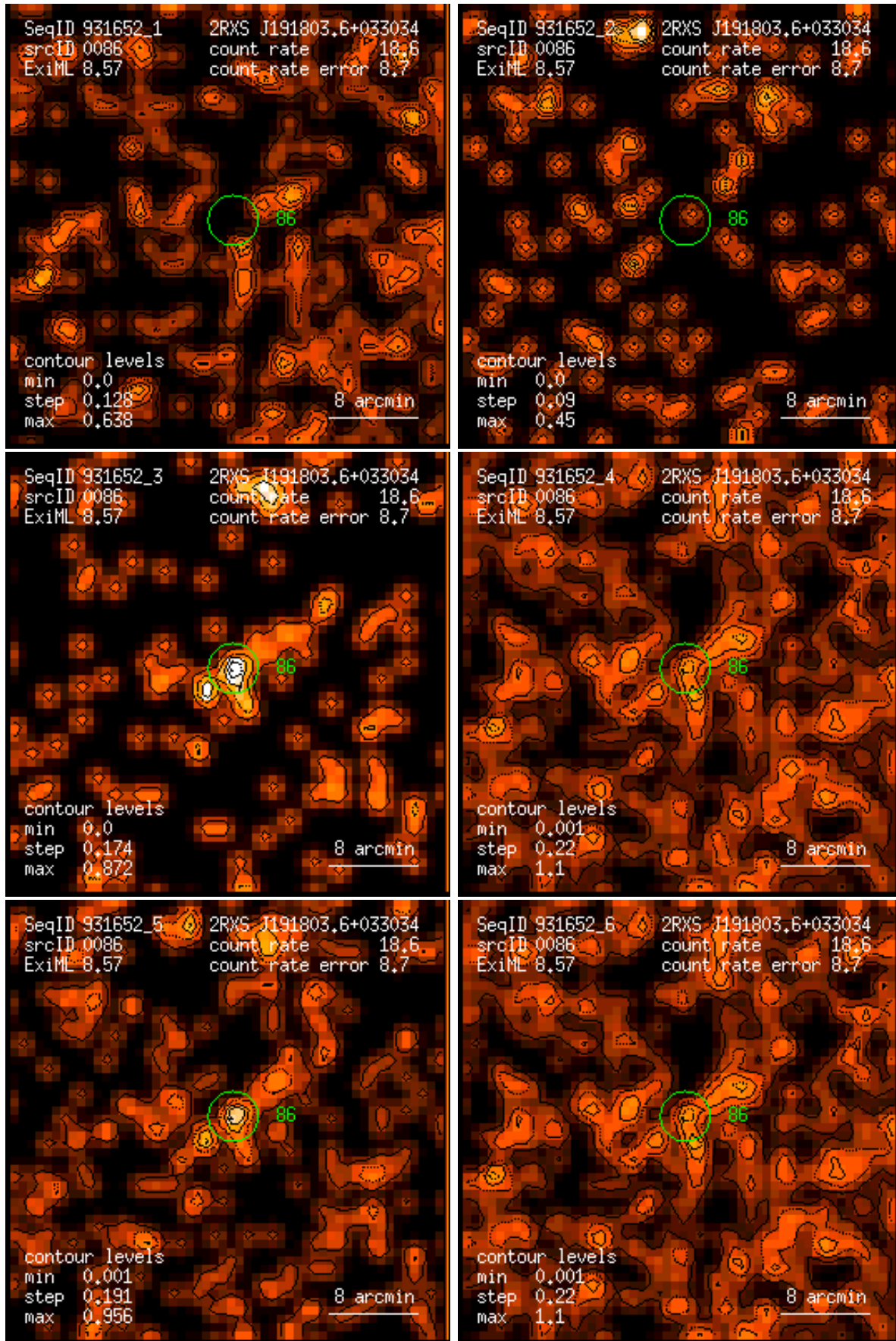
Figure 86: RASS 931652: detection 0086: band rate images, Gaussian filter: (1) PSPC channels 11 – 41, (2) 52 – 90, (3) 91 – 201, (4) 11 – 235, (5) 52 – 201, (6) 11 – 201. Broad band rates in counts/ks. Band rate contour levels in counts/ks/arcmin 2 .
