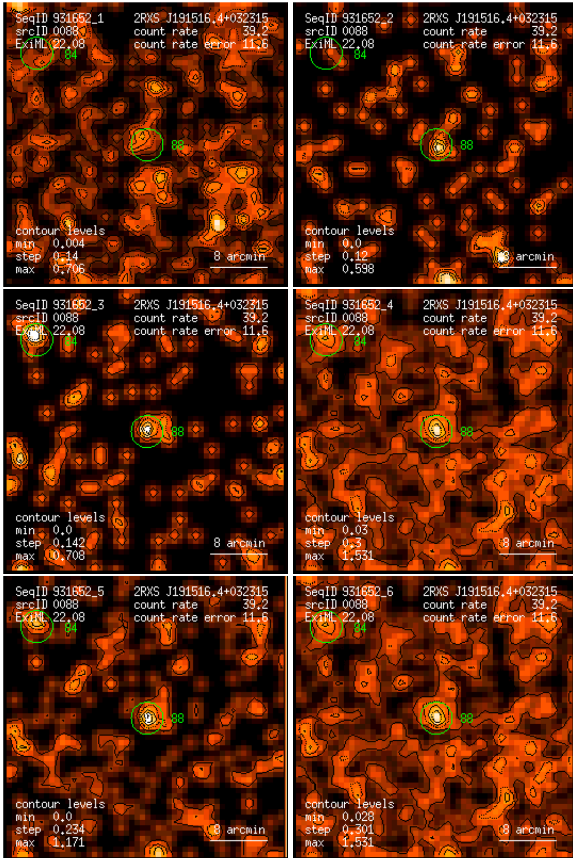
Figure 88: RASS 931652: detection 0088: band rate images, Gaussian filter: (1) PSPC channels 11 – 41, (2) 52 – 90, (3) 91 – 201, (4) 11 – 235, (5) 52 – 201, (6) 11 – 201. Broad band rates in counts/ks. Band rate contour levels in counts/ks/arcmin 2 .
