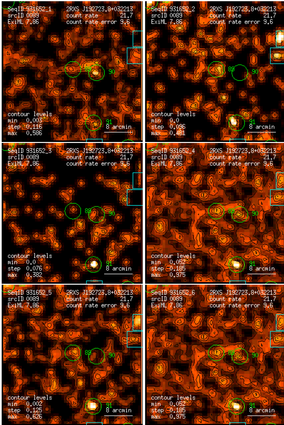
Figure 89: RASS 931652: detection 0089: band rate images, Gaussian filter: (1) PSPC channels 11 – 41, (2) 52 – 90, (3) 91 – 201, (4) 11 – 235, (5) 52 – 201, (6) 11 – 201. Broad band rates in counts/ks. Band rate contour levels in counts/ks/arcmin 2 .
