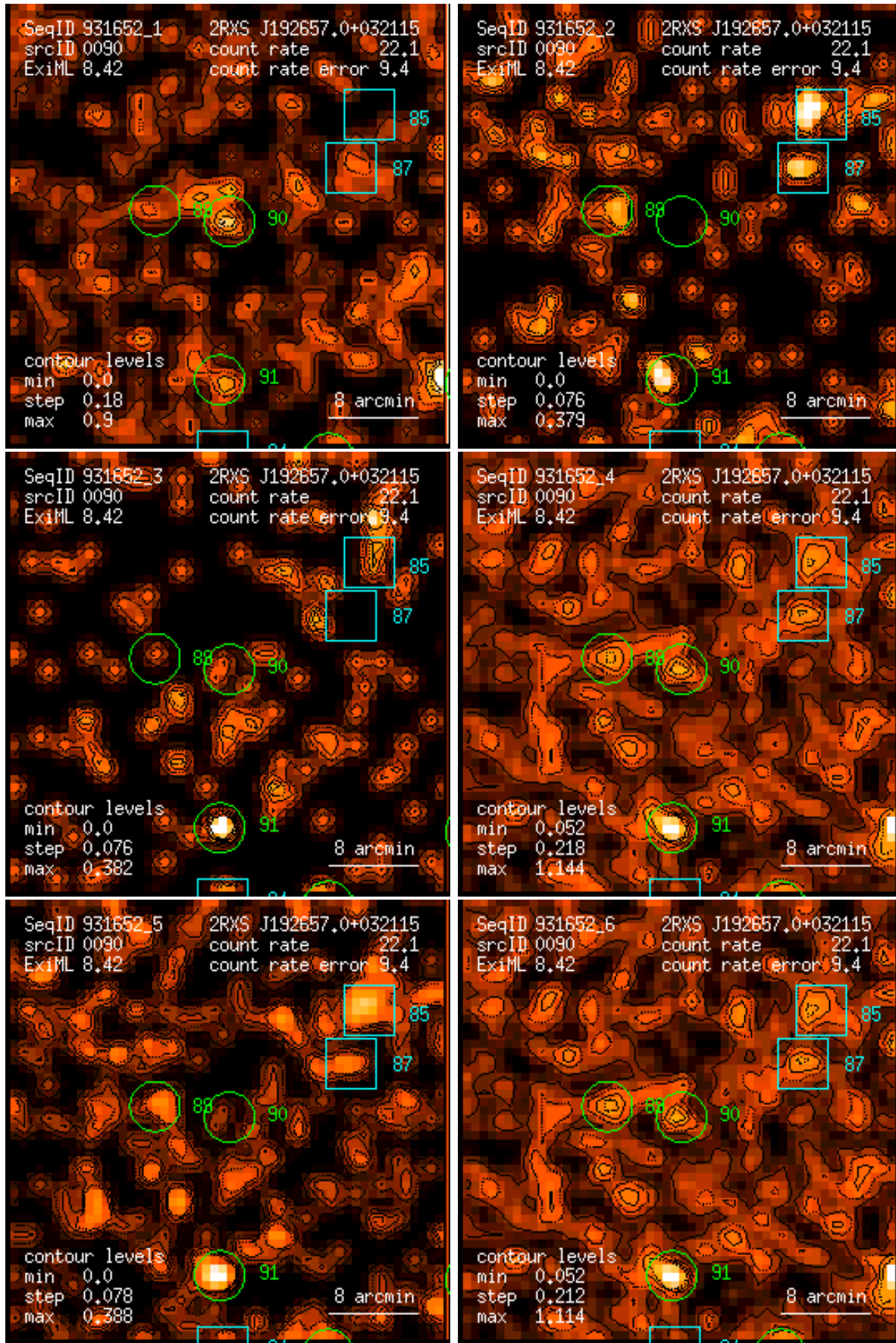
Figure 90: RASS 931652: detection 0090: band rate images, Gaussian filter: (1) PSPC channels 11 – 41, (2) 52 – 90, (3) 91 – 201, (4) 11 – 235, (5) 52 – 201, (6) 11 – 201. Broad band rates in counts/ks. Band rate contour levels in counts/ks/arcmin 2 .
