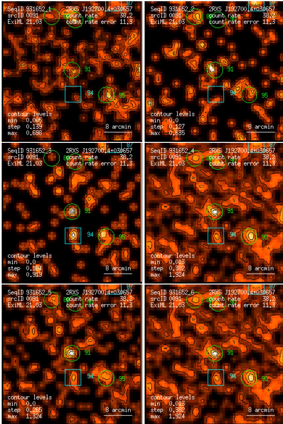
Figure 91: RASS 931652: detection 0091: band rate images, Gaussian filter: (1) PSPC channels 11 – 41, (2) 52 – 90, (3) 91 – 201, (4) 11 – 235, (5) 52 – 201, (6) 11 – 201. Broad band rates in counts/ks. Band rate contour levels in counts/ks/arcmin 2 .
