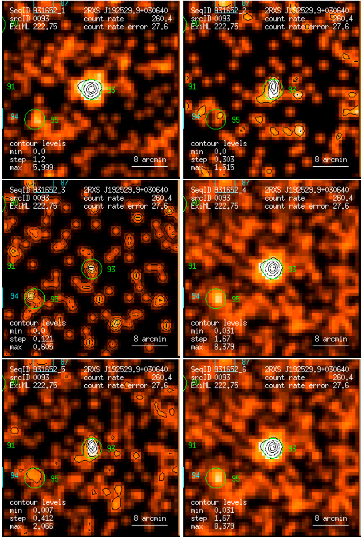
Figure 93: RASS 931652: detection 0093: band rate images, Gaussian filter: (1) PSPC channels 11 – 41, (2) 52 – 90, (3) 91 – 201, (4) 11 – 235, (5) 52 – 201, (6) 11 – 201. Broad band rates in counts/ks. Band rate contour levels in counts/ks/arcmin 2 .
