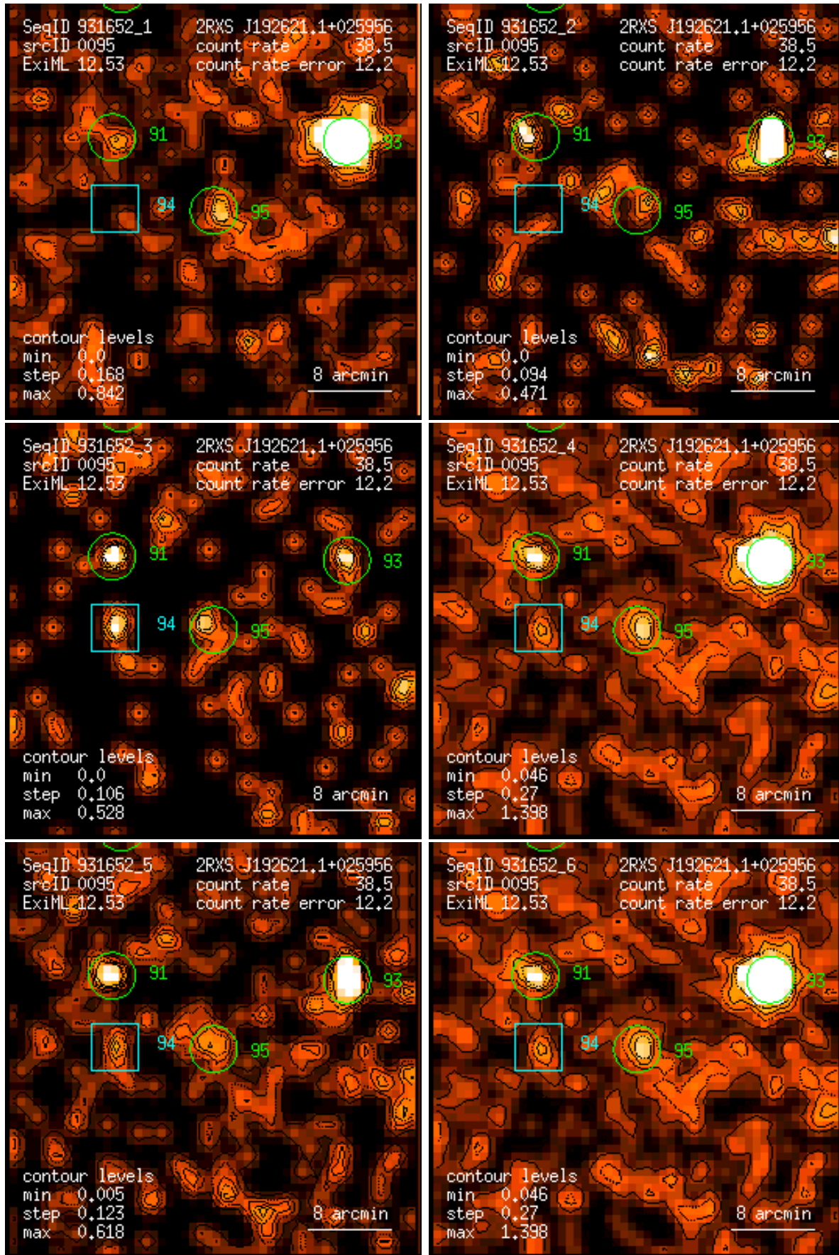
Figure 95: RASS 931652: detection 0095: band rate images, Gaussian filter: (1) PSPC channels 11 – 41, (2) 52 – 90, (3) 91 – 201, (4) 11 – 235, (5) 52 – 201, (6) 11 – 201. Broad band rates in counts/ks. Band rate contour levels in counts/ks/arcmin 2 .
