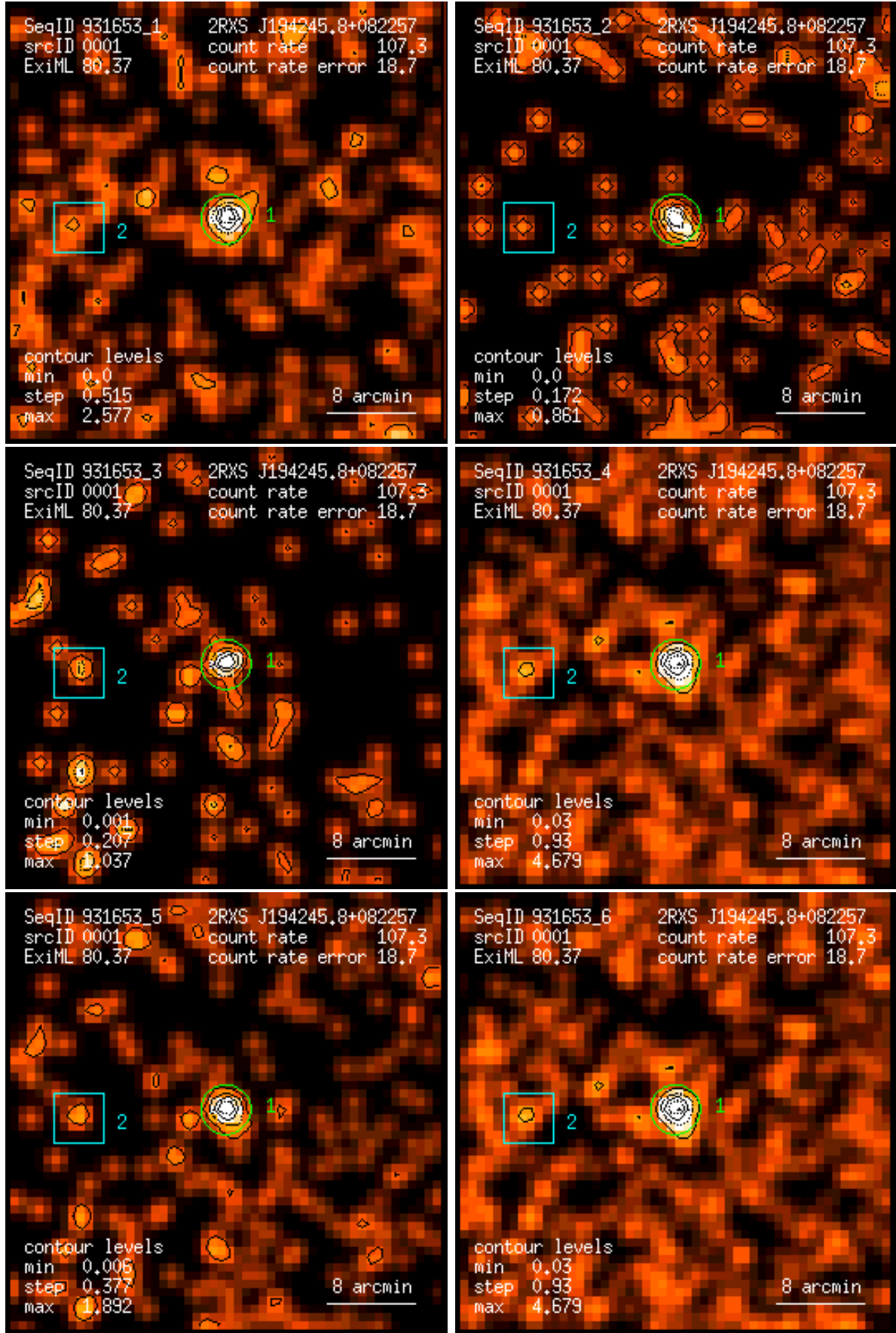
Figure 1: RASS 931653: detection 0001: band rate images, Gaussian filter: (1) PSPC channels 11 – 41, (2) 52 – 90, (3) 91 – 201, (4) 11 – 235, (5) 52 – 201, (6) 11 – 201. Broad band rates in counts/ks. Band rate contour levels in counts/ks/arcmin 2 .
