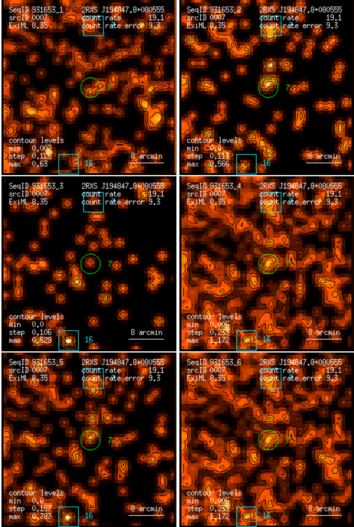
Figure 7: RASS 931653: detection 0007: band rate images, Gaussian filter: (1) PSPC channels 11 – 41, (2) 52 – 90, (3) 91 – 201, (4) 11 – 235, (5) 52 – 201, (6) 11 – 201. Broad band rates in counts/ks. Band rate contour levels in counts/ks/arcmin 2 .
