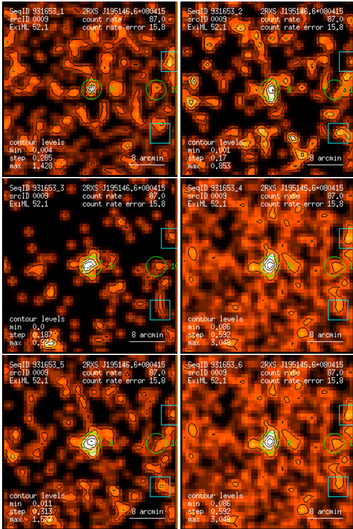
Figure 9: RASS 931653: detection 0009: band rate images, Gaussian filter: (1) PSPC channels 11 – 41, (2) 52 – 90, (3) 91 – 201, (4) 11 – 235, (5) 52 – 201, (6) 11 – 201. Broad band rates in counts/ks. Band rate contour levels in counts/ks/arcmin 2 .
