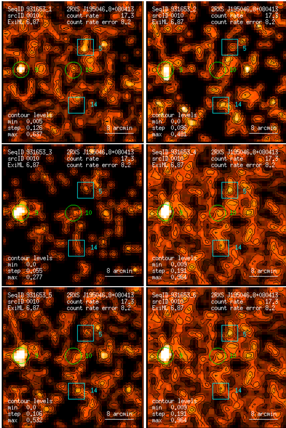
Figure 10: RASS 931653: detection 0010: band rate images, Gaussian filter: (1) PSPC channels 11 – 41, (2) 52 – 90, (3) 91 – 201, (4) 11 – 235, (5) 52 – 201, (6) 11 – 201. Broad band rates in counts/ks. Band rate contour levels in counts/ks/arcmin 2 .
