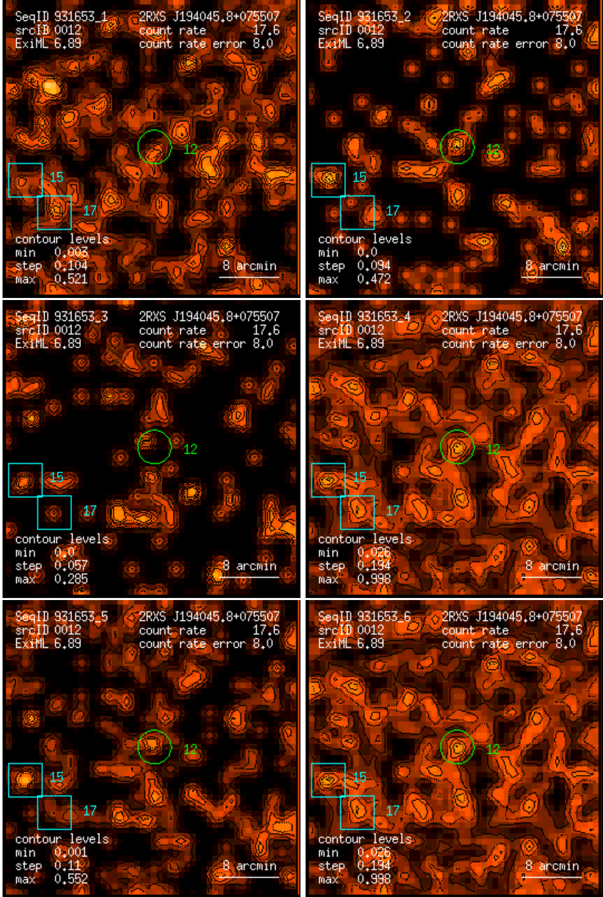
Figure 12: RASS 931653: detection 0012: band rate images, Gaussian filter: (1) PSPC channels 11 – 41, (2) 52 – 90, (3) 91 – 201, (4) 11 – 235, (5) 52 – 201, (6) 11 – 201. Broad band rates in counts/ks. Band rate contour levels in counts/ks/arcmin 2 .
