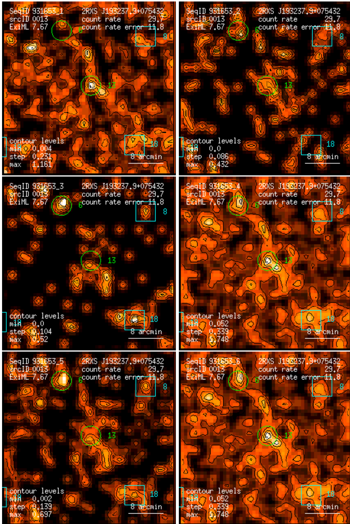
Figure 13: RASS 931653: detection 0013: band rate images, Gaussian filter: (1) PSPC channels 11 – 41, (2) 52 – 90, (3) 91 – 201, (4) 11 – 235, (5) 52 – 201, (6) 11 – 201. Broad band rates in counts/ks. Band rate contour levels in counts/ks/arcmin 2 .
