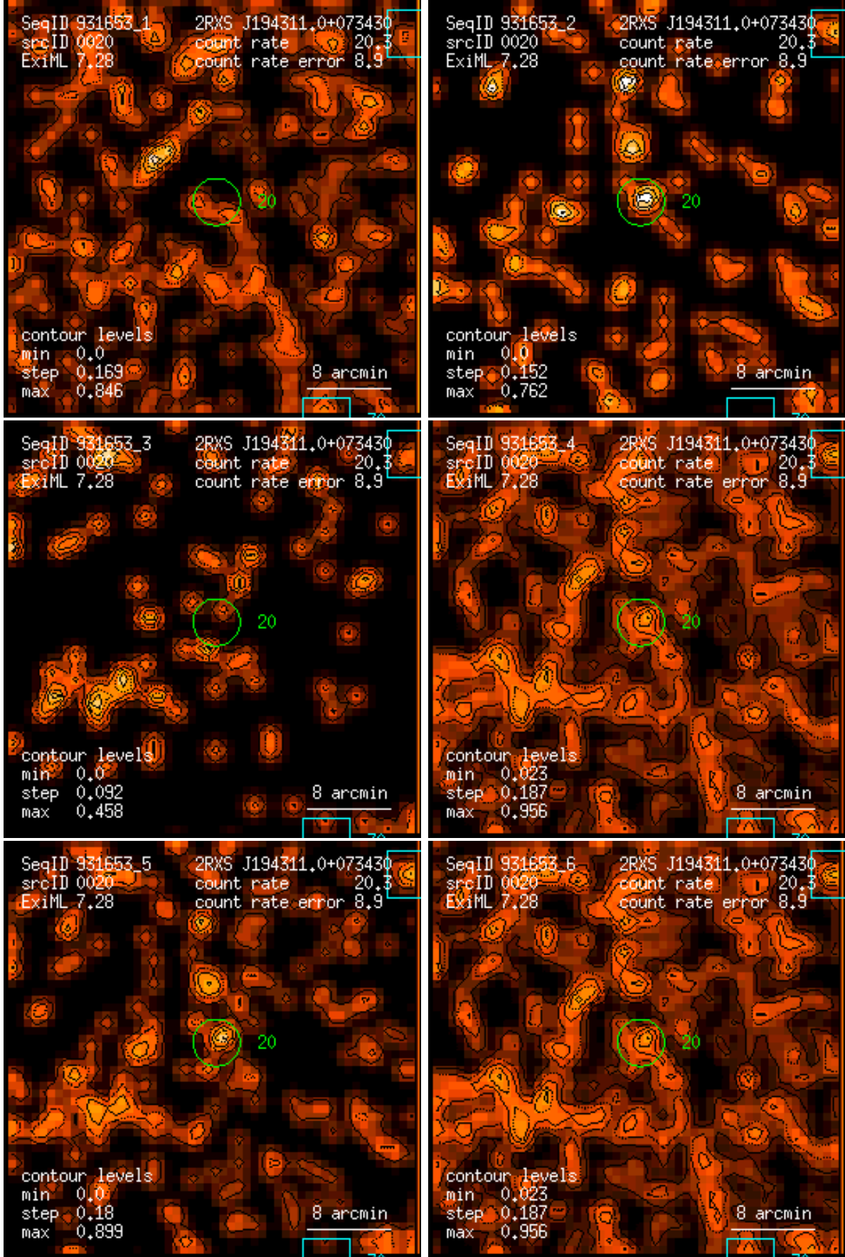
Figure 20: RASS 931653: detection 0020: band rate images, Gaussian filter: (1) PSPC channels 11 – 41, (2) 52 – 90, (3) 91 – 201, (4) 11 – 235, (5) 52 – 201, (6) 11 – 201. Broad band rates in counts/ks. Band rate contour levels in counts/ks/arcmin 2 .
