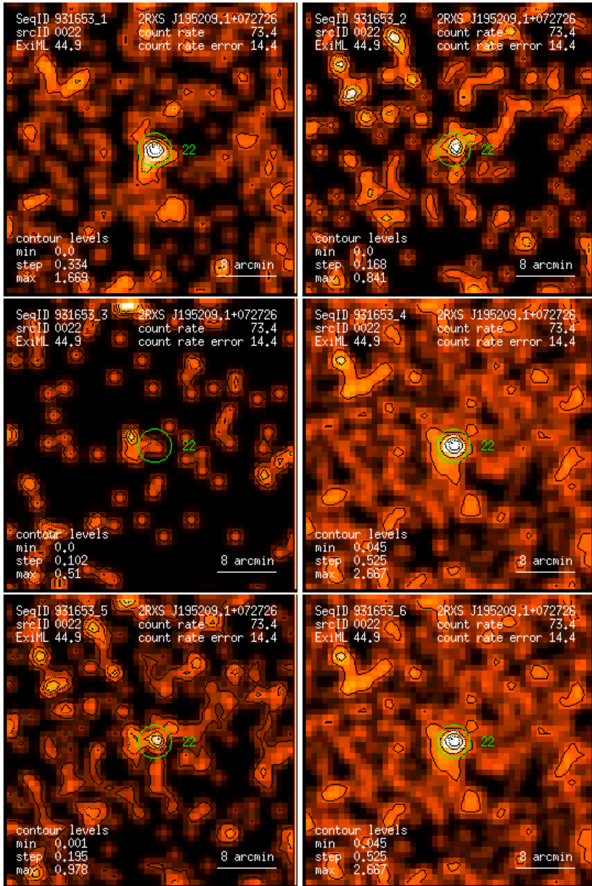
Figure 22: RASS 931653: detection 0022: band rate images, Gaussian filter: (1) PSPC channels 11 – 41, (2) 52 – 90, (3) 91 – 201, (4) 11 – 235, (5) 52 – 201, (6) 11 – 201. Broad band rates in counts/ks. Band rate contour levels in counts/ks/arcmin 2 .
