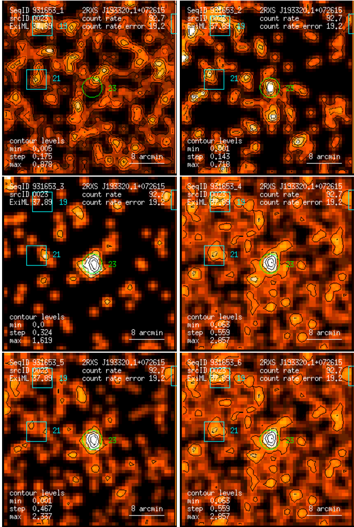
Figure 23: RASS 931653: detection 0023: band rate images, Gaussian filter: (1) PSPC channels 11 – 41, (2) 52 – 90, (3) 91 – 201, (4) 11 – 235, (5) 52 – 201, (6) 11 – 201. Broad band rates in counts/ks. Band rate contour levels in counts/ks/arcmin 2 .
