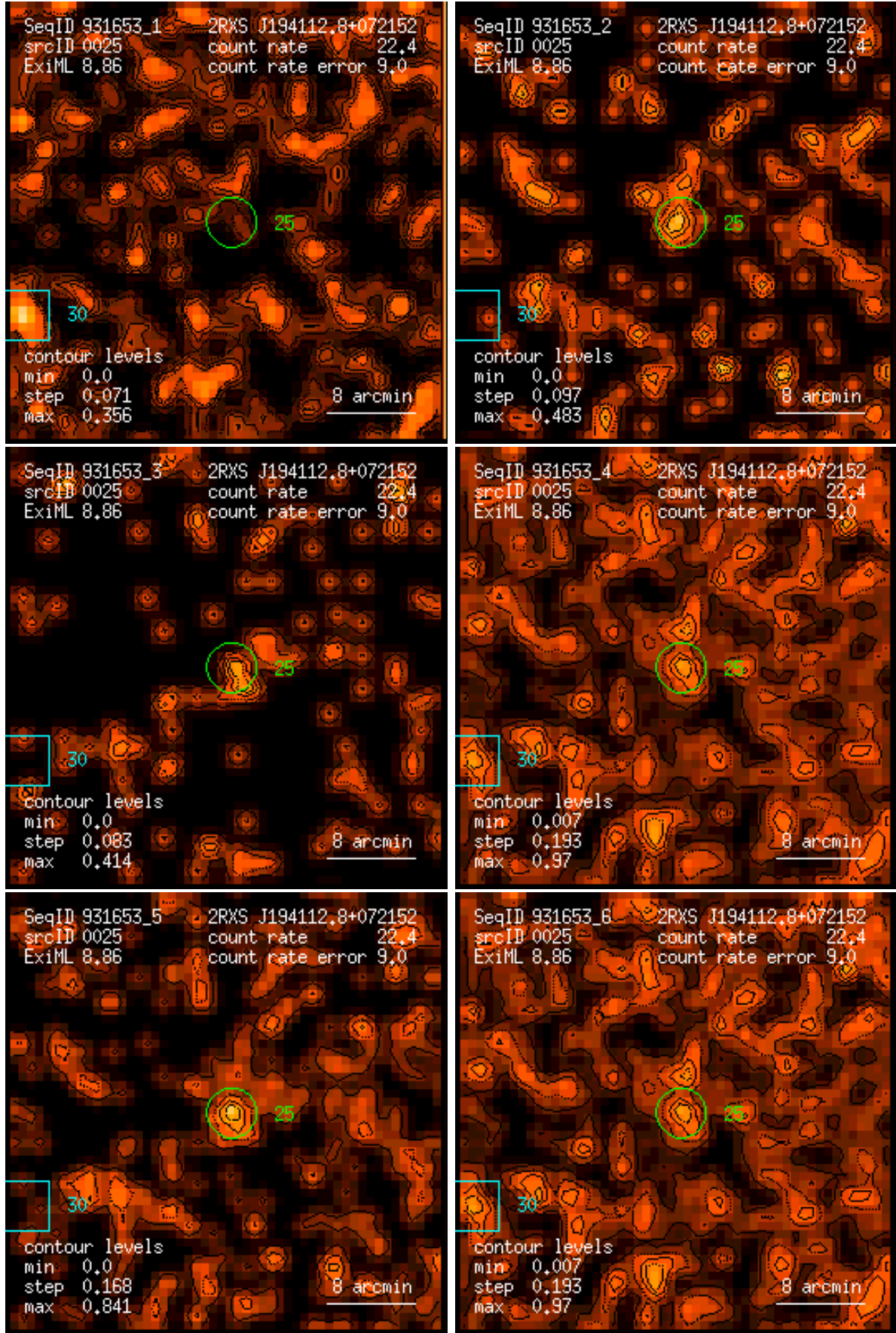
Figure 25: RASS 931653: detection 0025: band rate images, Gaussian filter: (1) PSPC channels 11 – 41, (2) 52 – 90, (3) 91 – 201, (4) 11 – 235, (5) 52 – 201, (6) 11 – 201. Broad band rates in counts/ks. Band rate contour levels in counts/ks/arcmin 2 .
