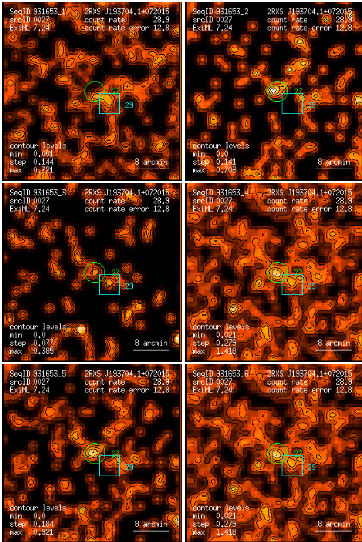
Figure 27: RASS 931653: detection 0027: band rate images, Gaussian filter: (1) PSPC channels 11 – 41, (2) 52 – 90, (3) 91 – 201, (4) 11 – 235, (5) 52 – 201, (6) 11 – 201. Broad band rates in counts/ks. Band rate contour levels in counts/ks/arcmin 2 .
