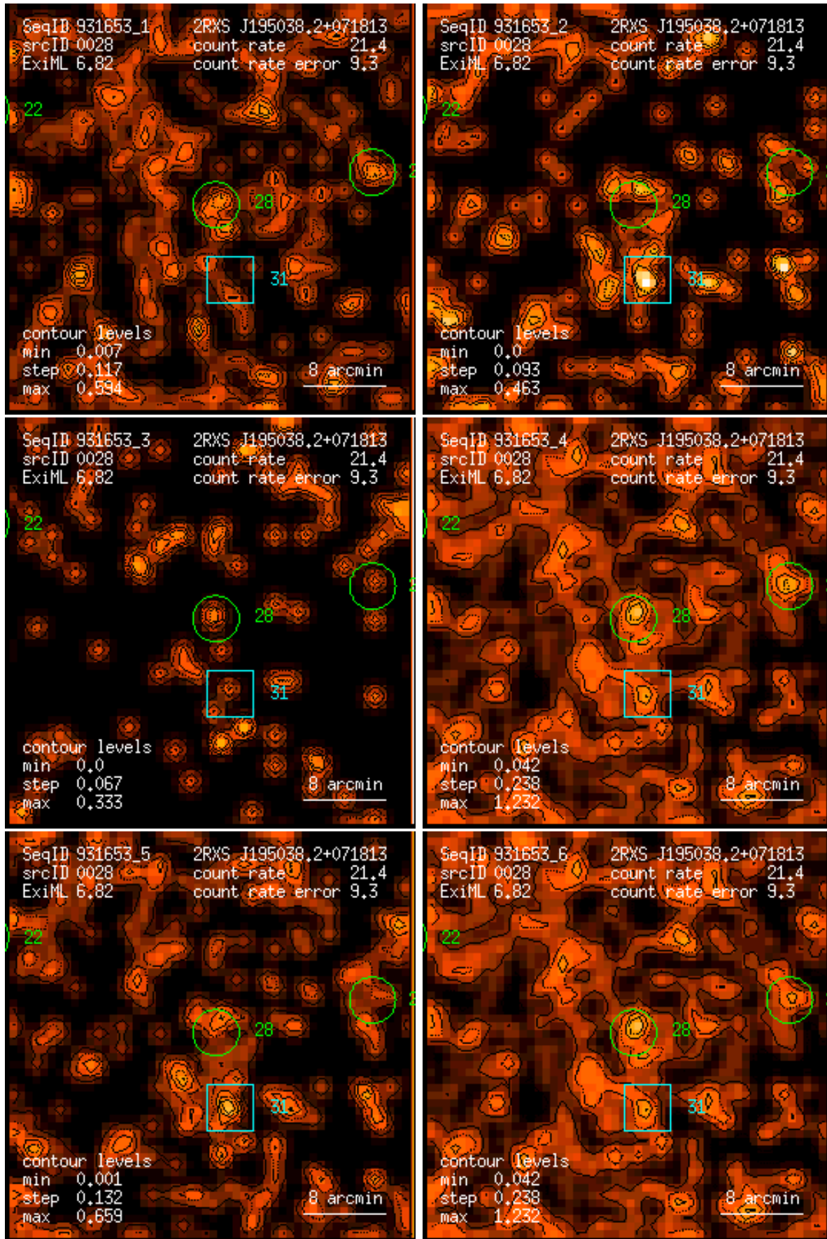
Figure 28: RASS 931653: detection 0028: band rate images, Gaussian filter: (1) PSPC channels 11 – 41, (2) 52 – 90, (3) 91 – 201, (4) 11 – 235, (5) 52 – 201, (6) 11 – 201. Broad band rates in counts/ks. Band rate contour levels in counts/ks/arcmin 2 .
