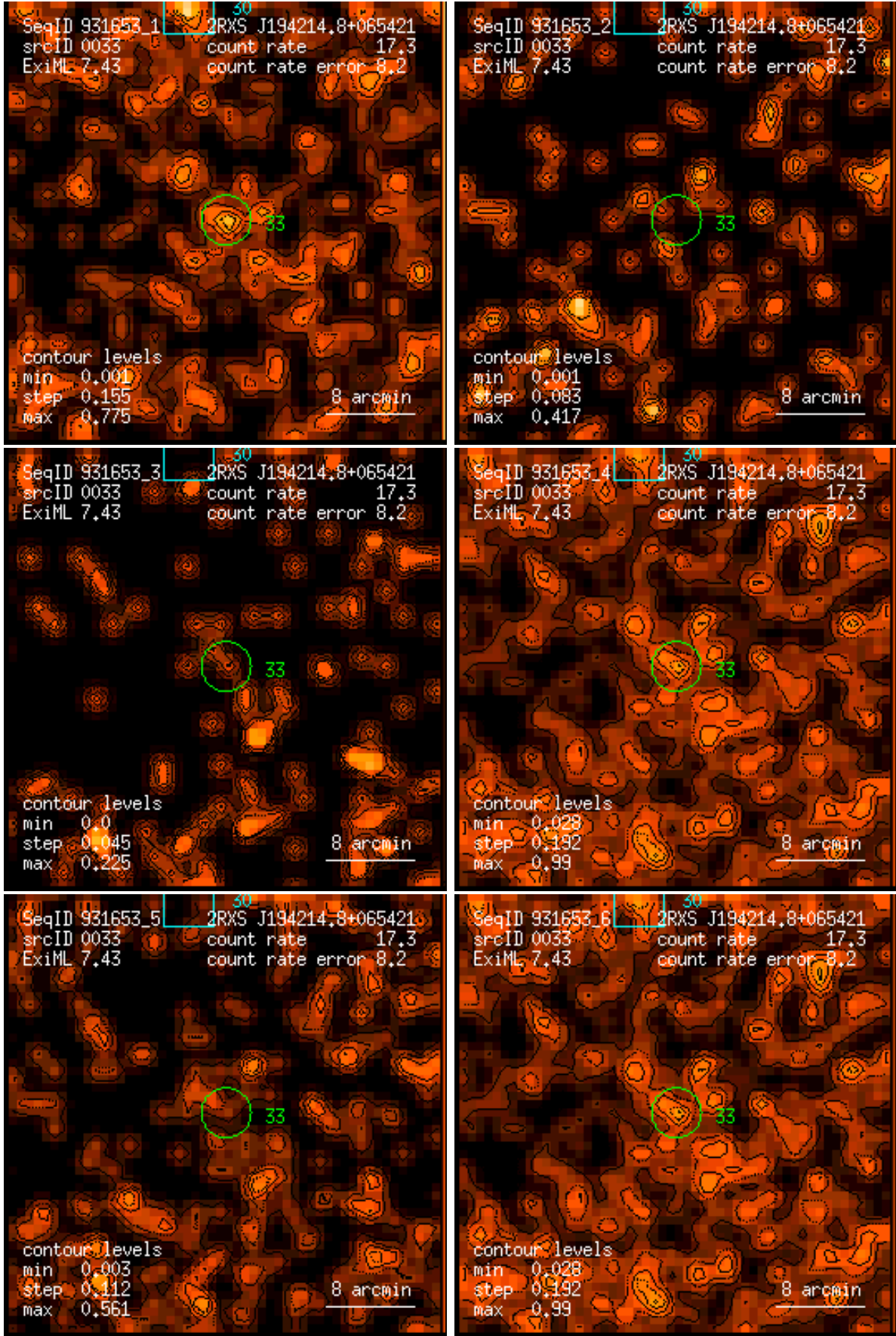
Figure 33: RASS 931653: detection 0033: band rate images, Gaussian filter: (1) PSPC channels 11 – 41, (2) 52 – 90, (3) 91 – 201, (4) 11 – 235, (5) 52 – 201, (6) 11 – 201. Broad band rates in counts/ks. Band rate contour levels in counts/ks/arcmin 2 .
