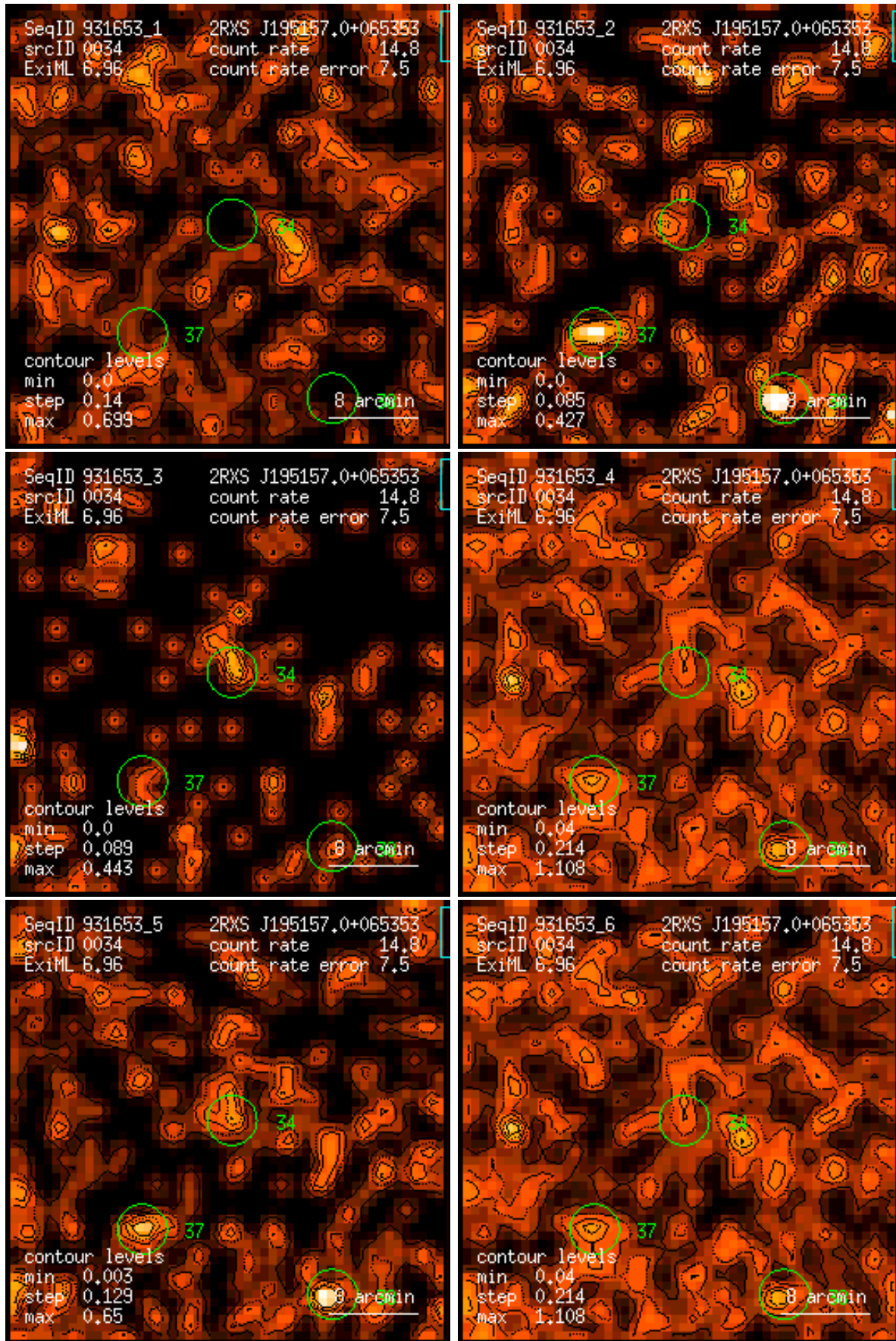
Figure 34: RASS 931653: detection 0034: band rate images, Gaussian filter: (1) PSPC channels 11 – 41, (2) 52 – 90, (3) 91 – 201, (4) 11 – 235, (5) 52 – 201, (6) 11 – 201. Broad band rates in counts/ks. Band rate contour levels in counts/ks/arcmin 2 .
