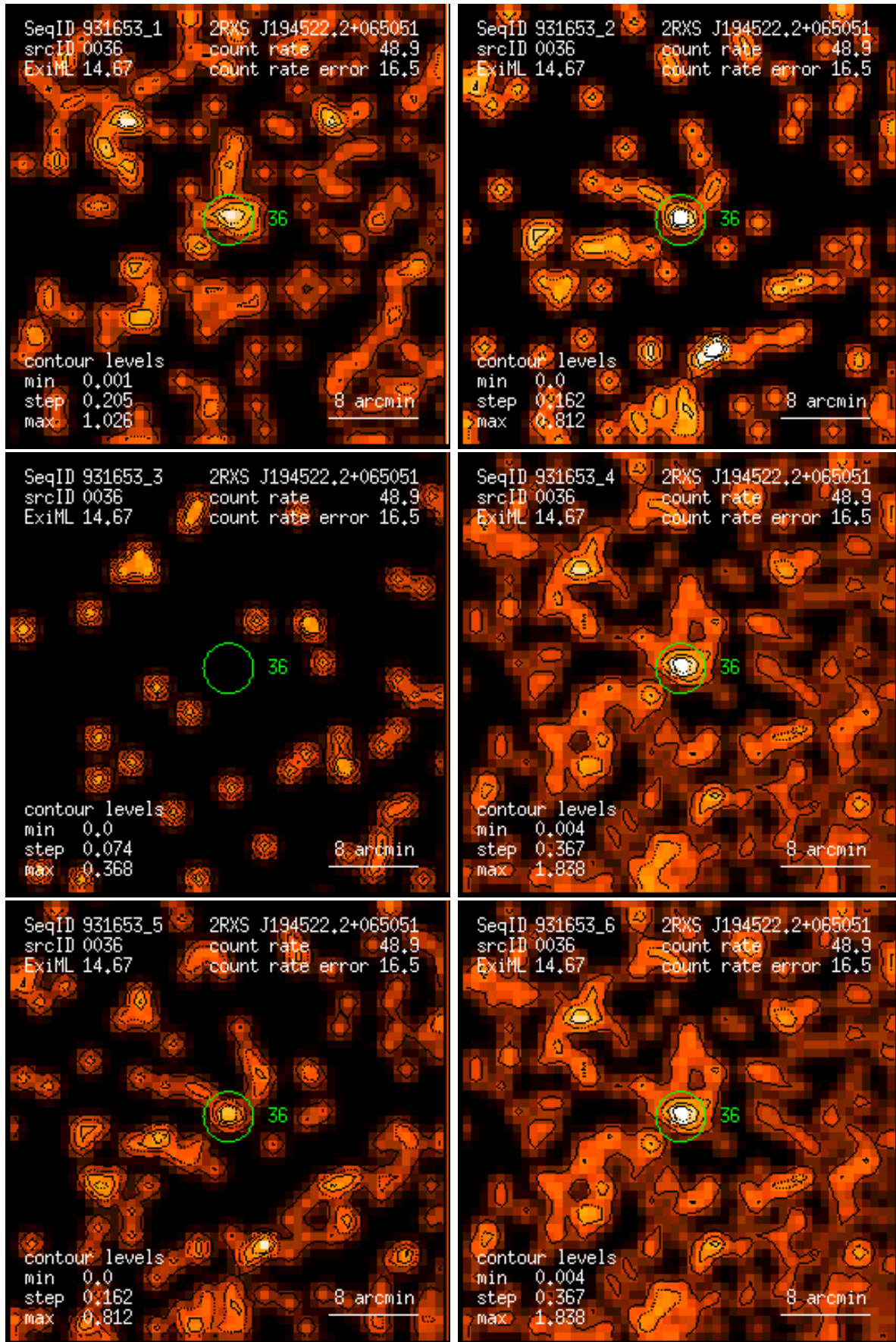
Figure 36: RASS 931653: detection 0036: band rate images, Gaussian filter: (1) PSPC channels 11 – 41, (2) 52 – 90, (3) 91 – 201, (4) 11 – 235, (5) 52 – 201, (6) 11 – 201. Broad band rates in counts/ks. Band rate contour levels in counts/ks/arcmin 2 .
