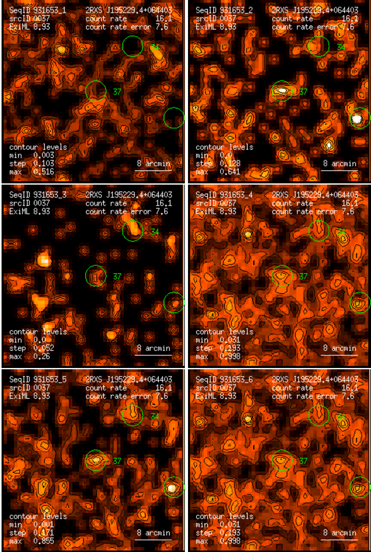
Figure 37: RASS 931653: detection 0037: band rate images, Gaussian filter: (1) PSPC channels 11 – 41, (2) 52 – 90, (3) 91 – 201, (4) 11 – 235, (5) 52 – 201, (6) 11 – 201. Broad band rates in counts/ks. Band rate contour levels in counts/ks/arcmin 2 .
