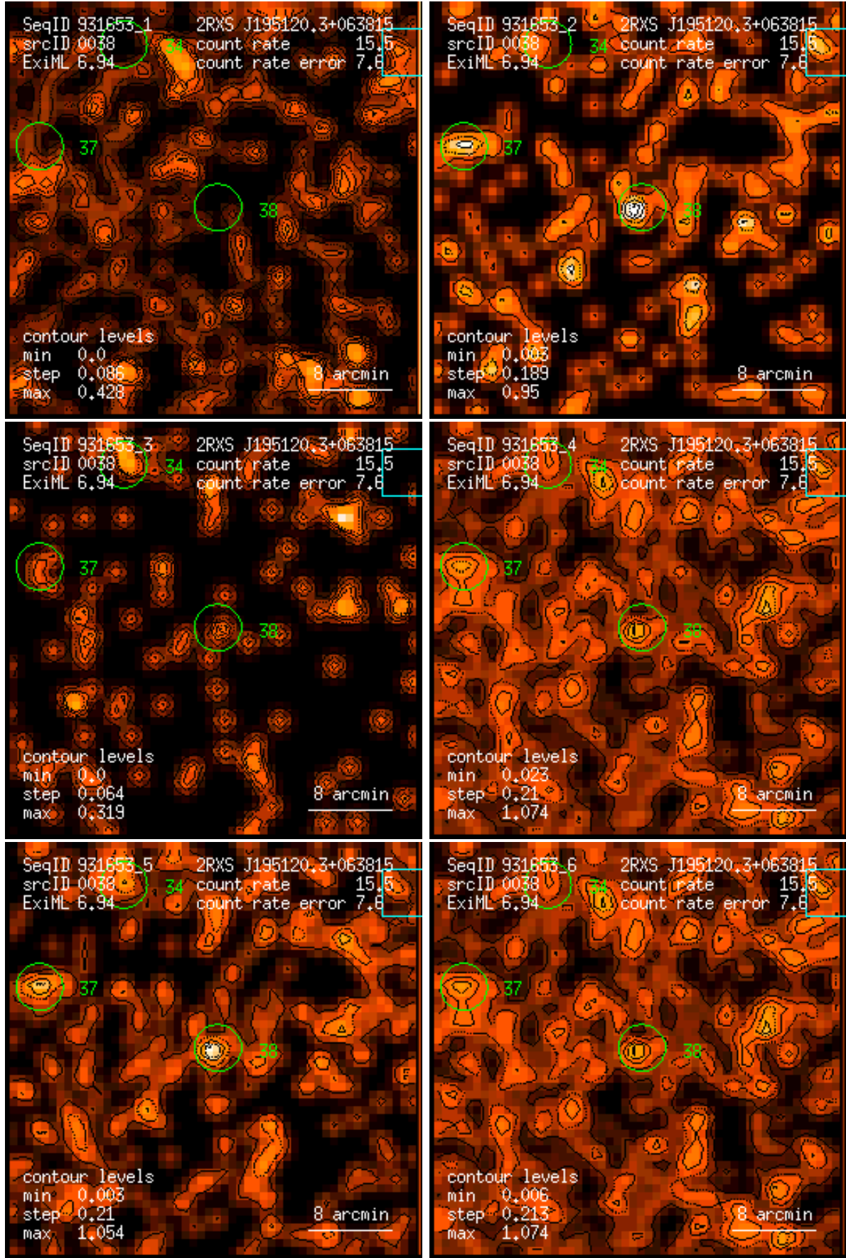
Figure 38: RASS 931653: detection 0038: band rate images, Gaussian filter: (1) PSPC channels 11 – 41, (2) 52 – 90, (3) 91 – 201, (4) 11 – 235, (5) 52 – 201, (6) 11 – 201. Broad band rates in counts/ks. Band rate contour levels in counts/ks/arcmin 2 .
