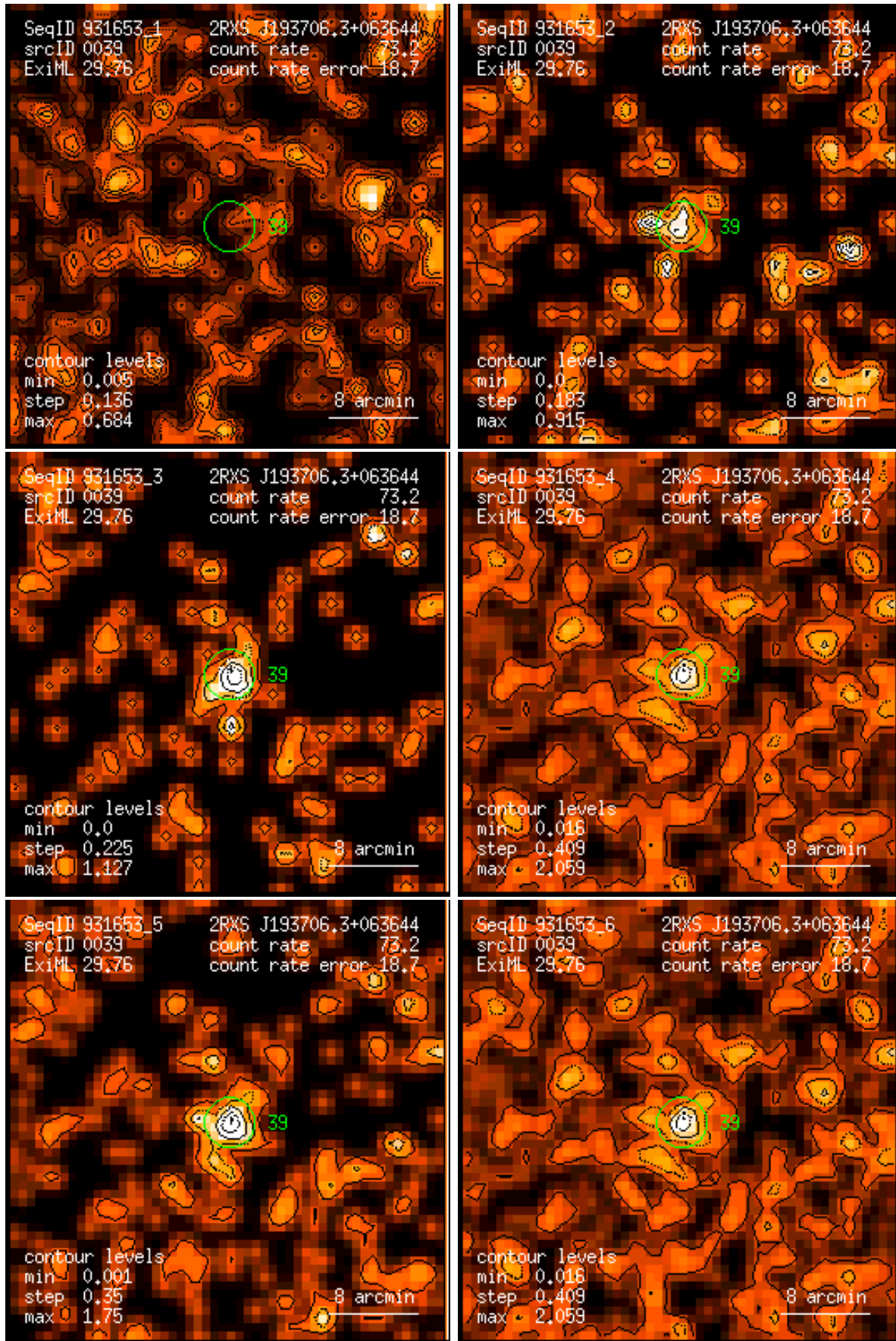
Figure 39: RASS 931653: detection 0039: band rate images, Gaussian filter: (1) PSPC channels 11 – 41, (2) 52 – 90, (3) 91 – 201, (4) 11 – 235, (5) 52 – 201, (6) 11 – 201. Broad band rates in counts/ks. Band rate contour levels in counts/ks/arcmin 2 .
