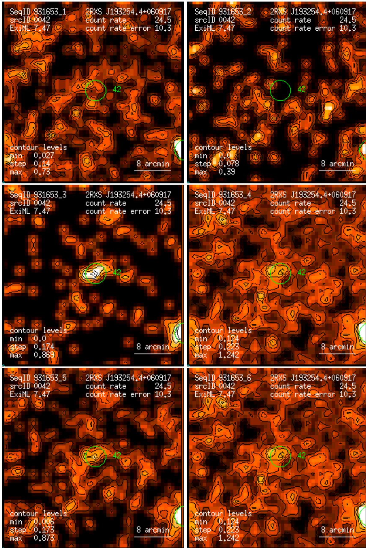
Figure 42: RASS 931653: detection 0042: band rate images, Gaussian filter: (1) PSPC channels 11 – 41, (2) 52 – 90, (3) 91 – 201, (4) 11 – 235, (5) 52 – 201, (6) 11 – 201. Broad band rates in counts/ks. Band rate contour levels in counts/ks/arcmin 2 .
