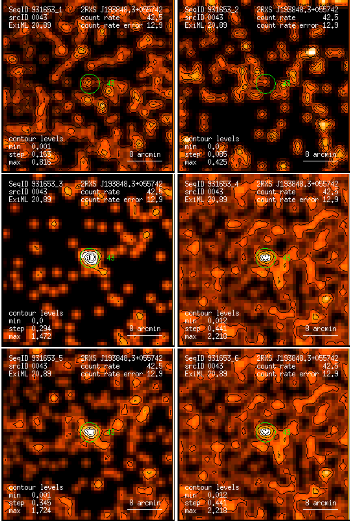
Figure 43: RASS 931653: detection 0043: band rate images, Gaussian filter: (1) PSPC channels 11 – 41, (2) 52 – 90, (3) 91 – 201, (4) 11 – 235, (5) 52 – 201, (6) 11 – 201. Broad band rates in counts/ks. Band rate contour levels in counts/ks/arcmin 2 .
