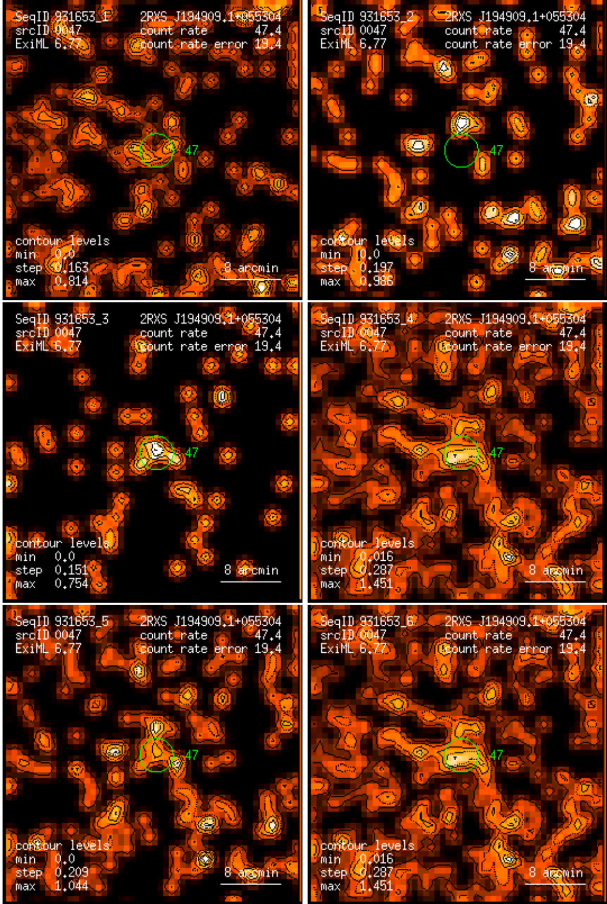
Figure 47: RASS 931653: detection 0047: band rate images, Gaussian filter: (1) PSPC channels 11 – 41, (2) 52 – 90, (3) 91 – 201, (4) 11 – 235, (5) 52 – 201, (6) 11 – 201. Broad band rates in counts/ks. Band rate contour levels in counts/ks/arcmin 2 .
