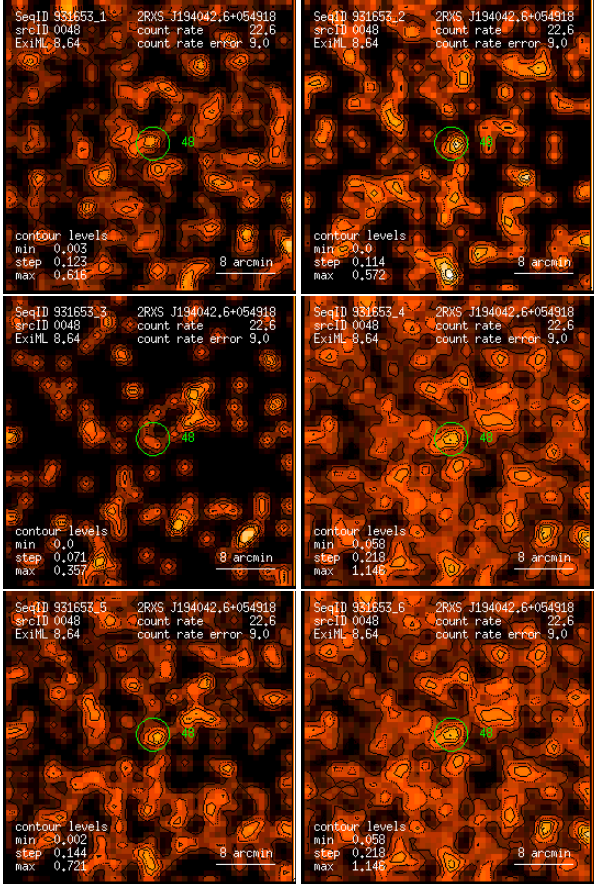
Figure 48: RASS 931653: detection 0048: band rate images, Gaussian filter: (1) PSPC channels 11 – 41, (2) 52 – 90, (3) 91 – 201, (4) 11 – 235, (5) 52 – 201, (6) 11 – 201. Broad band rates in counts/ks. Band rate contour levels in counts/ks/arcmin 2 .
