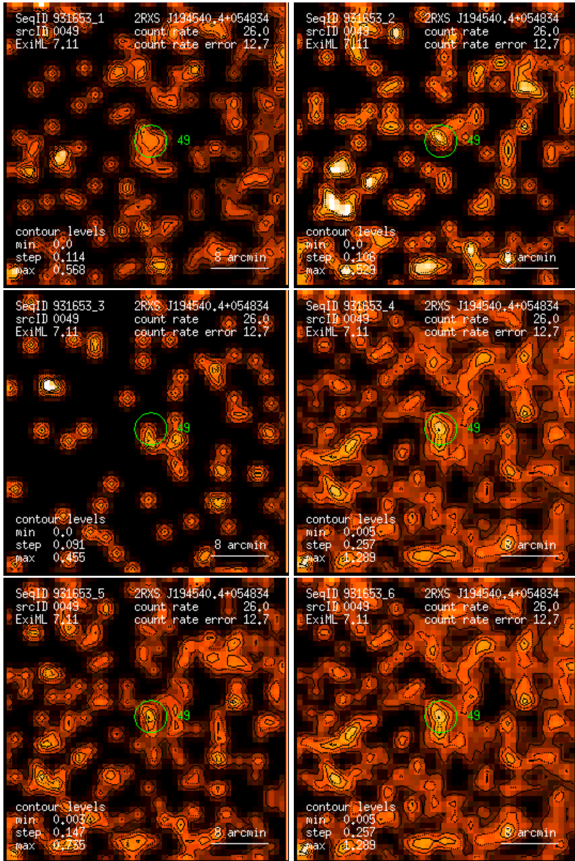
Figure 49: RASS 931653: detection 0049: band rate images, Gaussian filter: (1) PSPC channels 11 – 41, (2) 52 – 90, (3) 91 – 201, (4) 11 – 235, (5) 52 – 201, (6) 11 – 201. Broad band rates in counts/ks. Band rate contour levels in counts/ks/arcmin 2 .
