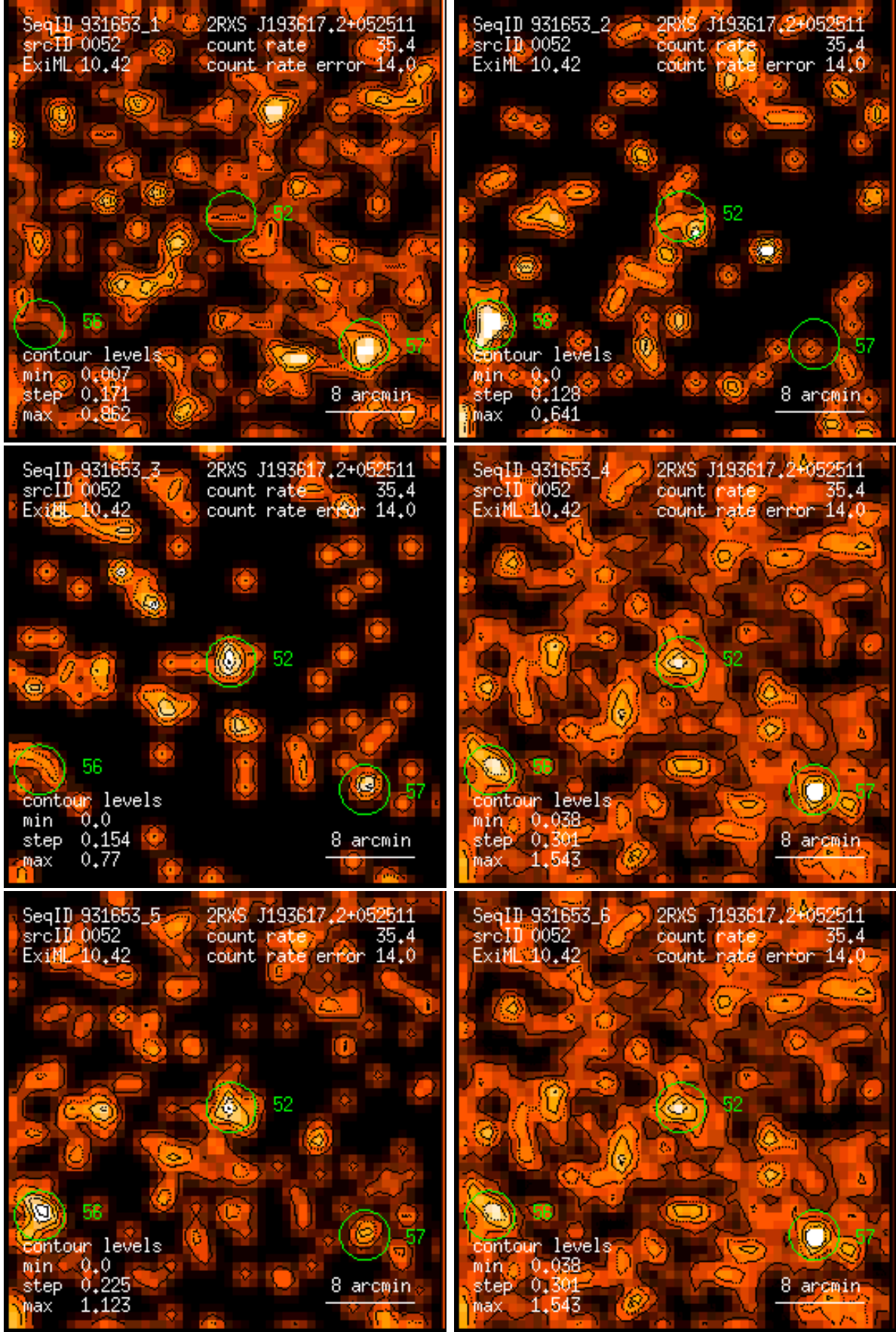
Figure 52: RASS 931653: detection 0052: band rate images, Gaussian filter: (1) PSPC channels 11 – 41, (2) 52 – 90, (3) 91 – 201, (4) 11 – 235, (5) 52 – 201, (6) 11 – 201. Broad band rates in counts/ks. Band rate contour levels in counts/ks/arcmin 2 .
