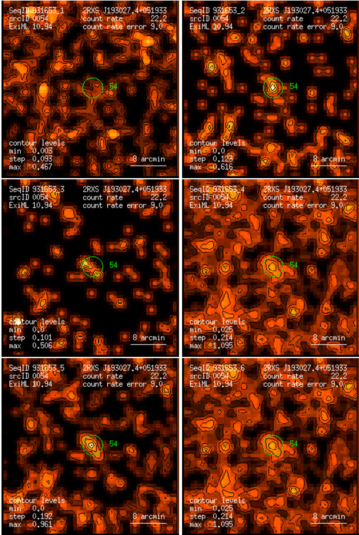
Figure 54: RASS 931653: detection 0054: band rate images, Gaussian filter: (1) PSPC channels 11 – 41, (2) 52 – 90, (3) 91 – 201, (4) 11 – 235, (5) 52 – 201, (6) 11 – 201. Broad band rates in counts/ks. Band rate contour levels in counts/ks/arcmin 2 .
