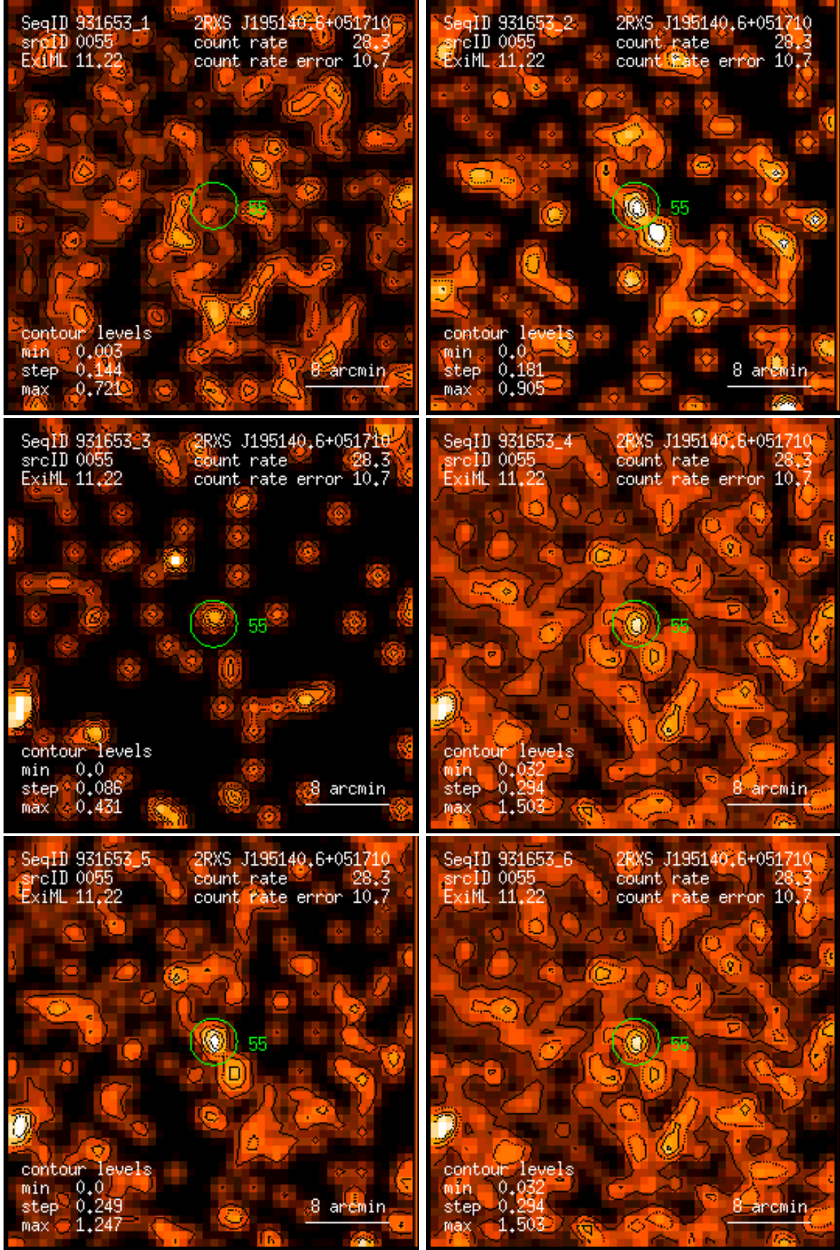
Figure 55: RASS 931653: detection 0055: band rate images, Gaussian filter: (1) PSPC channels 11 – 41, (2) 52 – 90, (3) 91 – 201, (4) 11 – 235, (5) 52 – 201, (6) 11 – 201. Broad band rates in counts/ks. Band rate contour levels in counts/ks/arcmin 2 .
