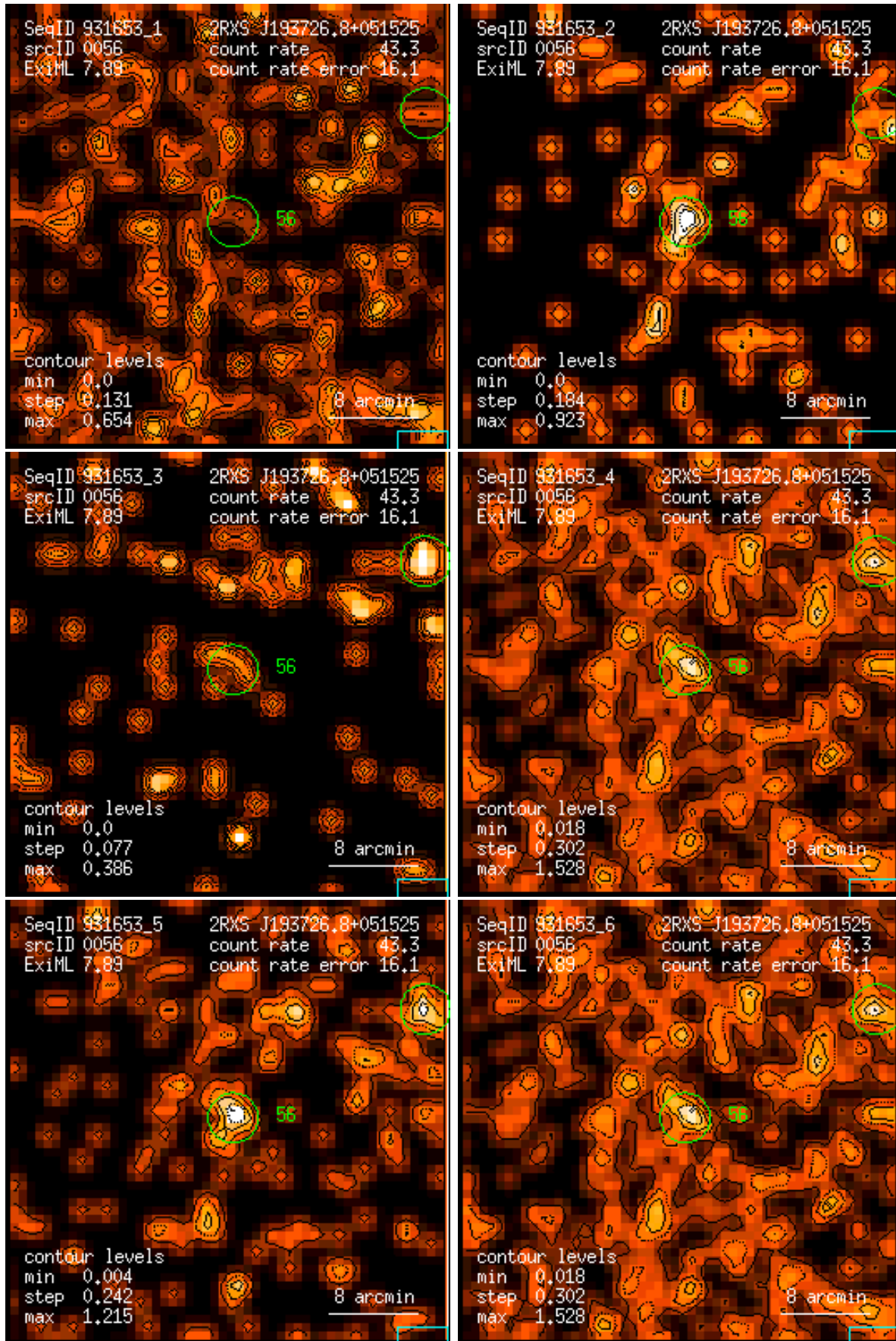
Figure 56: RASS 931653: detection 0056: band rate images, Gaussian filter: (1) PSPC channels 11 – 41, (2) 52 – 90, (3) 91 – 201, (4) 11 – 235, (5) 52 – 201, (6) 11 – 201. Broad band rates in counts/ks. Band rate contour levels in counts/ks/arcmin 2 .
