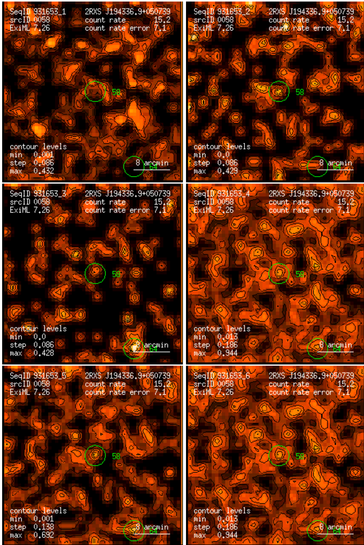
Figure 58: RASS 931653: detection 0058: band rate images, Gaussian filter: (1) PSPC channels 11 – 41, (2) 52 – 90, (3) 91 – 201, (4) 11 – 235, (5) 52 – 201, (6) 11 – 201. Broad band rates in counts/ks. Band rate contour levels in counts/ks/arcmin 2 .
