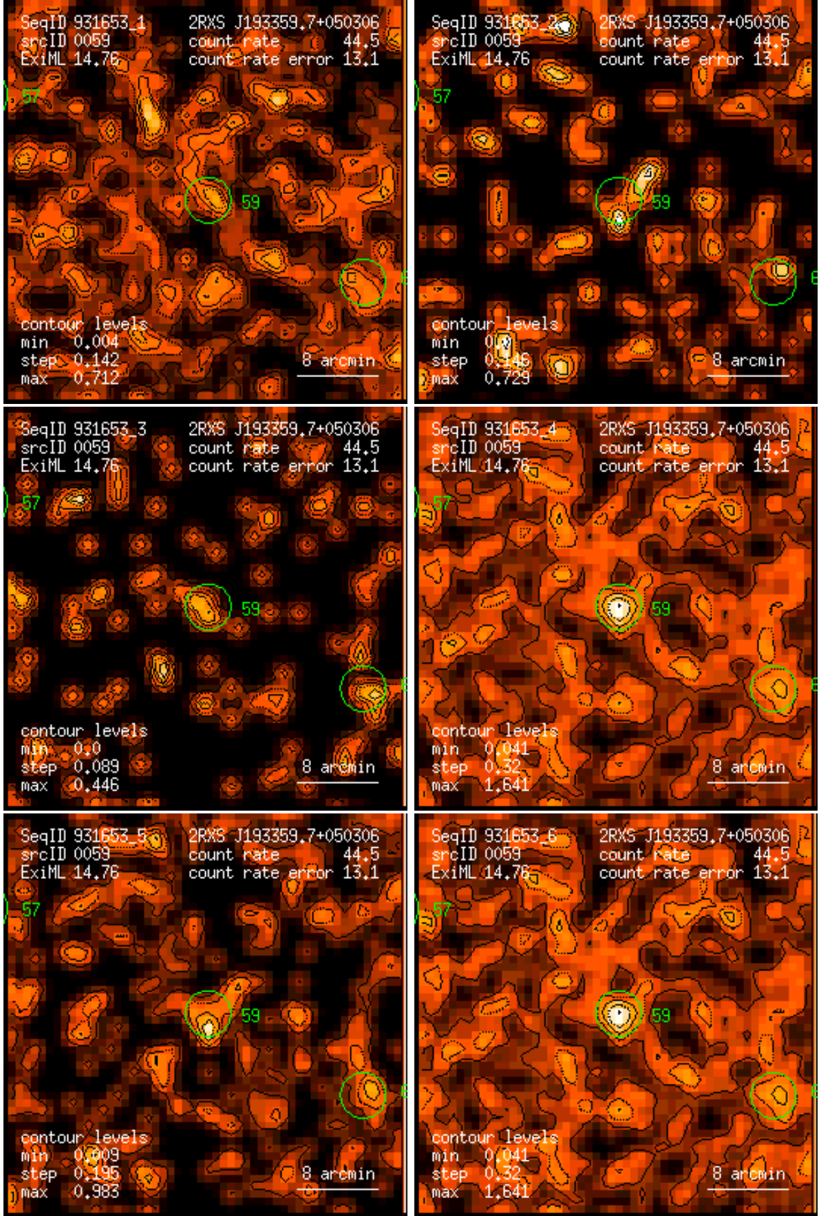
Figure 59: RASS 931653: detection 0059: band rate images, Gaussian filter: (1) PSPC channels 11 – 41, (2) 52 – 90, (3) 91 – 201, (4) 11 – 235, (5) 52 – 201, (6) 11 – 201. Broad band rates in counts/ks. Band rate contour levels in counts/ks/arcmin 2 .
